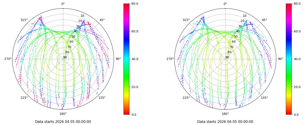
Skyplot for station LALA. Parameter M1C Data file LALA00ESP_R_2026095.xtr Skyplot for station LALA. Parameter M2C Data file LALA00ESP_R_2026095.xtr
