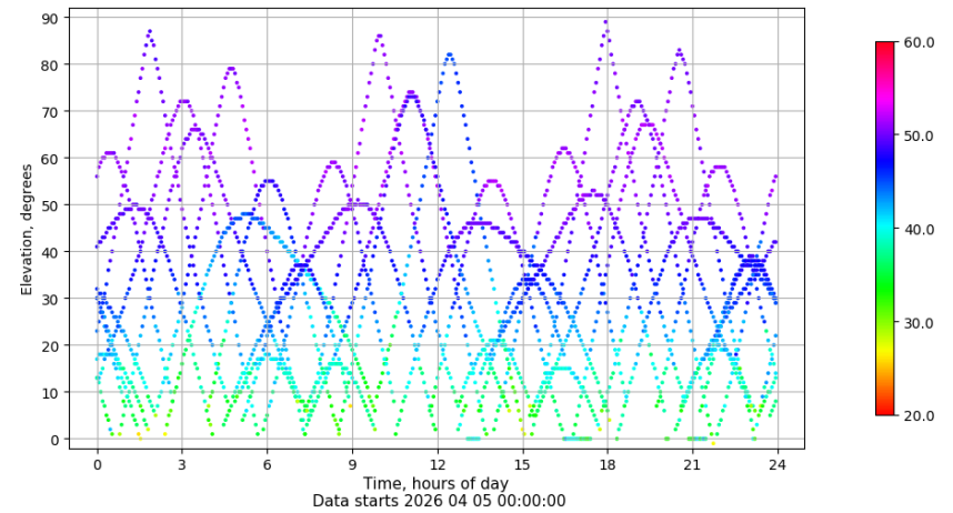
Time-elevation plot for station LALA. Signal to Noise S1C Data file LALA00ESP_R_2026095.xtr
