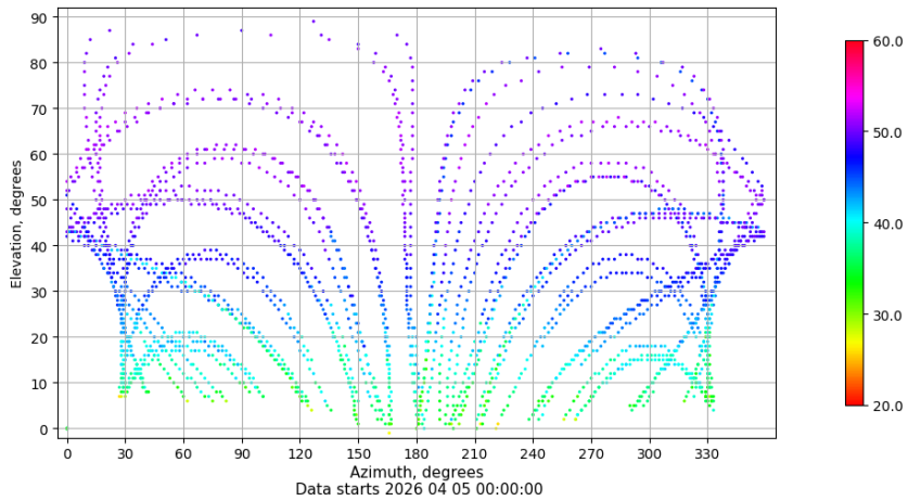
Azimuth-elevation plot for station LALA. Signal to Noise S1C Data file LALA00ESP_R_2026095.xtr
