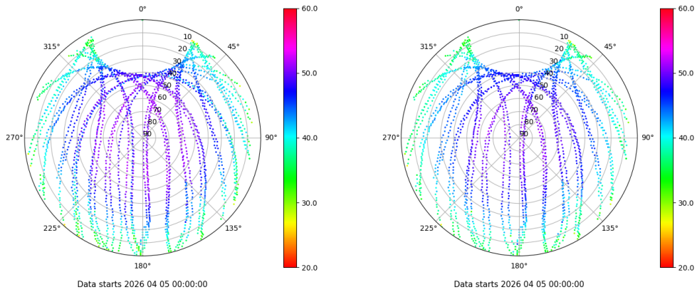
Skyplot for station LALA. Signal to Noise S1C Data file LALA00ESP_R_2026095.xtr Skyplot for station LALA. Signal to Noise S2C Data file LALA00ESP_R_2026095.xtr
