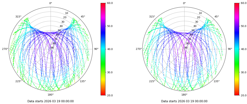
Skyplot for station LALA. Signal to Noise S1C Data file LALA00ESP_R_2026078.xtr Skyplot for station LALA. Signal to Noise S2X Data file LALA00ESP_R_2026078.xtr
