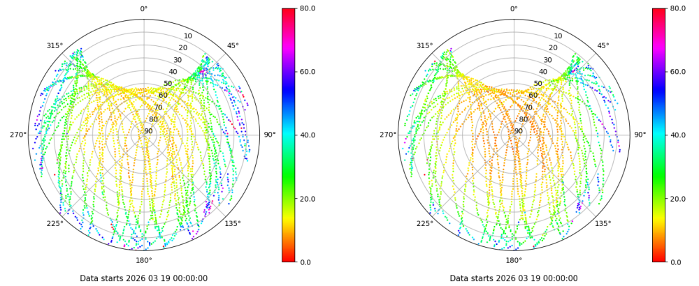
Skyplot for station LALA. Parameter M1C Data file LALA00ESP_R_2026078.xtr Skyplot for station LALA. Parameter M2X Data file LALA00ESP_R_2026078.xtr
