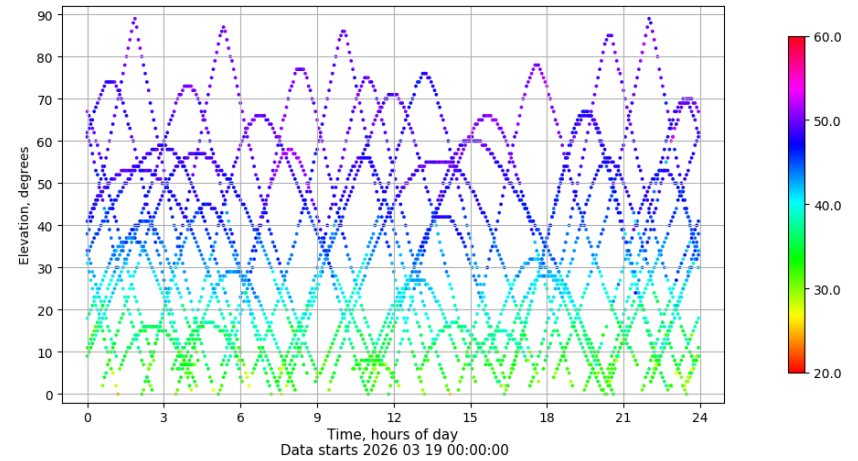
Time-elevation plot for station LALA. Signal to Noise S1C Data file LALA00ESP_R_2026078.xtr
