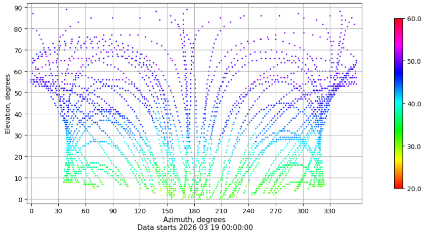
Azimuth-elevation plot for station LALA. Signal to Noise S1C Data file LALA00ESP_R_2026078.xtr
