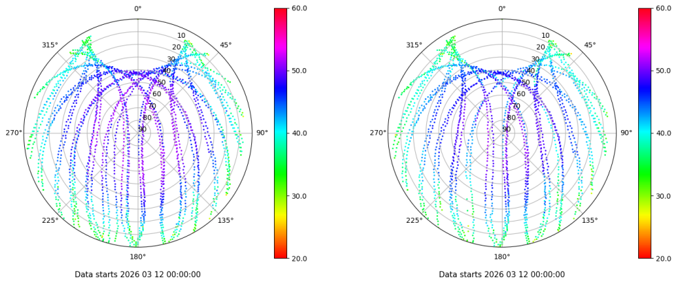
Skyplot for station LALA. Signal to Noise S1C Data file LALA00ESP_R_2026071.xtr Skyplot for station LALA. Signal to Noise S2C Data file LALA00ESP_R_2026071.xtr
