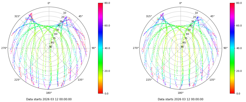
Skyplot for station LALA. Parameter M1C Data file LALA00ESP_R_2026071.xtr Skyplot for station LALA. Parameter M2C Data file LALA00ESP_R_2026071.xtr
