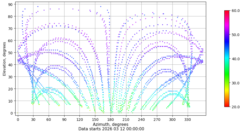
Azimuth-elevation plot for station LALA. Signal to Noise S1C Data file LALA00ESP_R_2026071.xtr
