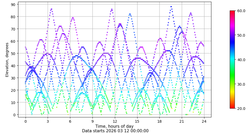
Time-elevation plot for station LALA. Signal to Noise S1C Data file LALA00ESP_R_2026071.xtr
