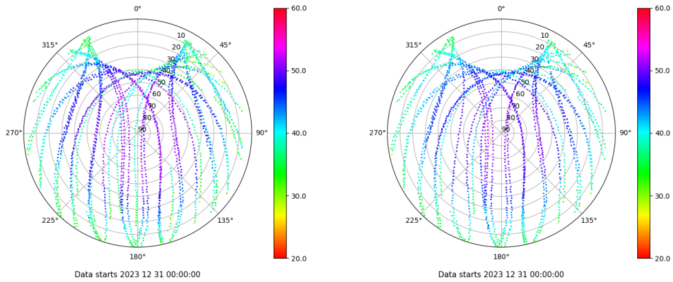
Skyplot for station LALA. Signal to Noise S1C Data file LALA00ESP_R_2023365.xtr Skyplot for station LALA. Signal to Noise S2C Data file LALA00ESP_R_2023365.xtr
