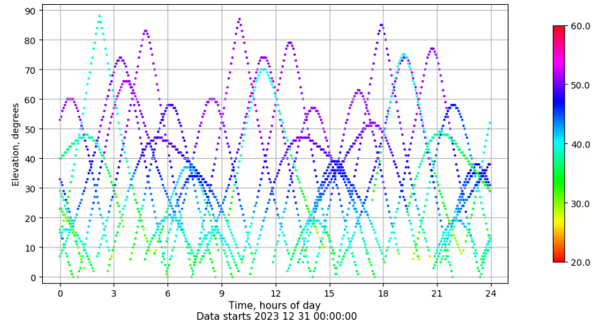
Time-elevation plot for station LALA. Signal to Noise S1C Data file LALA00ESP_R_2023365.xtr
