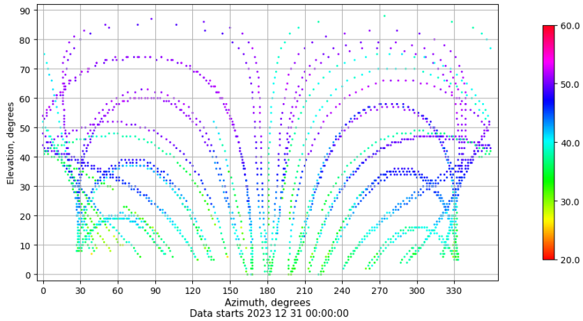
Azimuth-elevation plot for station LALA. Signal to Noise S1C Data file LALA00ESP_R_2023365.xtr
