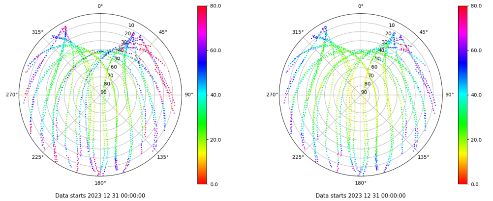
Skyplot for station LALA. Parameter M1C Data file LALA00ESP_R_2023365.xtr Skyplot for station LALA. Parameter M2C Data file LALA00ESP_R_2023365.xtr
