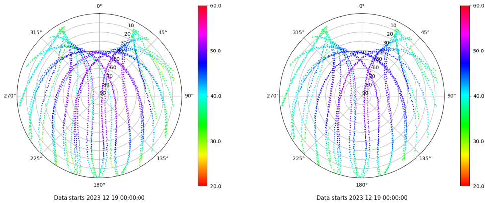
Skyplot for station LALA. Signal to Noise S1C Data file LALA00ESP_R_2023353.xtr Skyplot for station LALA. Signal to Noise S2C Data file LALA00ESP_R_2023353.xtr
