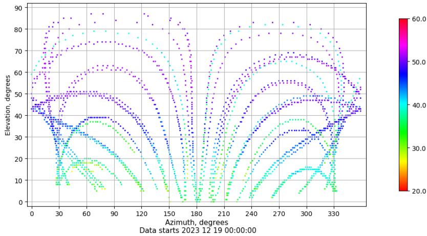
Azimuth-elevation plot for station LALA. Signal to Noise S1C Data file LALA00ESP_R_2023353.xtr
