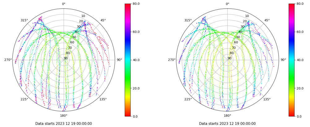
Skyplot for station LALA. Parameter M1C Data file LALA00ESP_R_2023353.xtr Skyplot for station LALA. Parameter M2C Data file LALA00ESP_R_2023353.xtr
