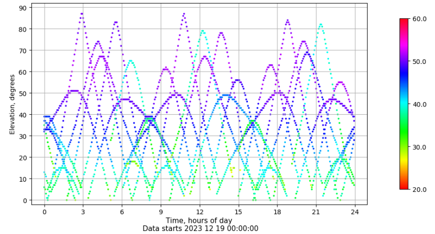
Time-elevation plot for station LALA. Signal to Noise S1C Data file LALA00ESP_R_2023353.xtr
