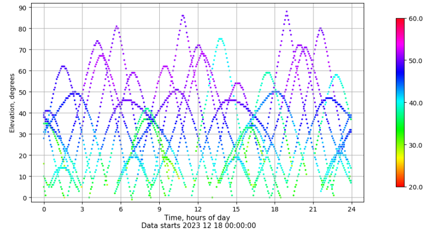
Time-elevation plot for station LALA. Signal to Noise S1C Data file LALA00ESP_R_2023352.xtr
