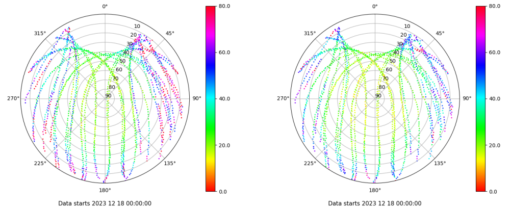
Skyplot for station LALA. Parameter M1C Data file LALA00ESP_R_2023352.xtr Skyplot for station LALA. Parameter M2C Data file LALA00ESP_R_2023352.xtr
