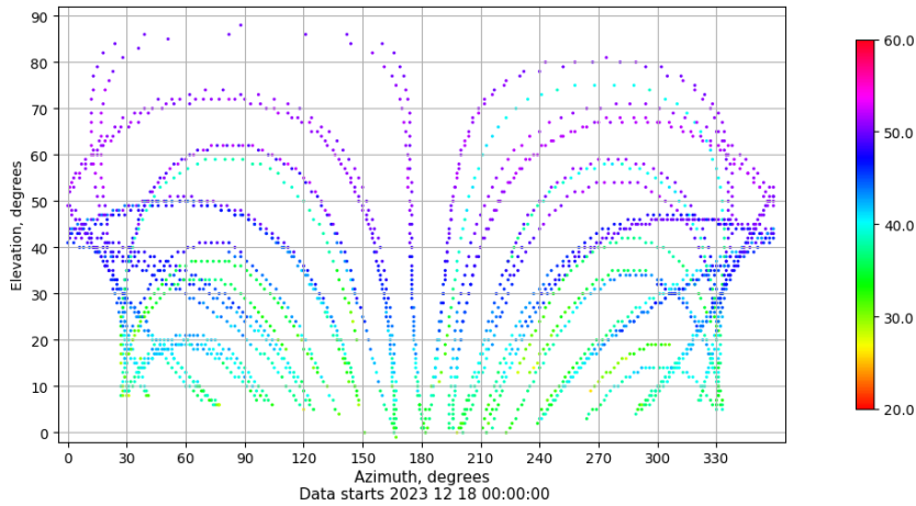
Azimuth-elevation plot for station LALA. Signal to Noise S1C Data file LALA00ESP_R_2023352.xtr
