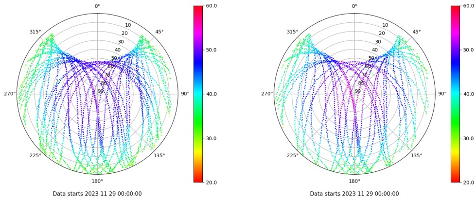
Skyplot for station LALA. Signal to Noise S1C Data file LALA00ESP_R_2023333.xtr Skyplot for station LALA. Signal to Noise S2X Data file LALA00ESP_R_2023333.xtr
