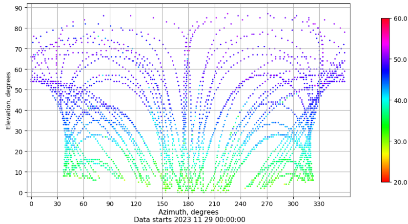
Azimuth-elevation plot for station LALA. Signal to Noise S1C Data file LALA00ESP_R_2023333.xtr
