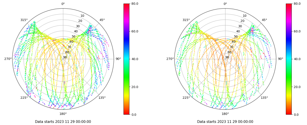
Skyplot for station LALA. Parameter M1C Data file LALA00ESP_R_2023333.xtr Skyplot for station LALA. Parameter M2X Data file LALA00ESP_R_2023333.xtr
