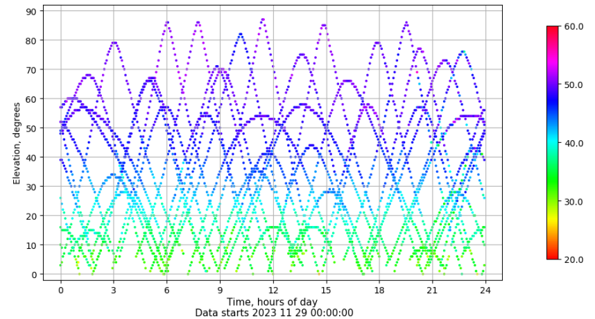
Time-elevation plot for station LALA. Signal to Noise S1C Data file LALA00ESP_R_2023333.xtr
