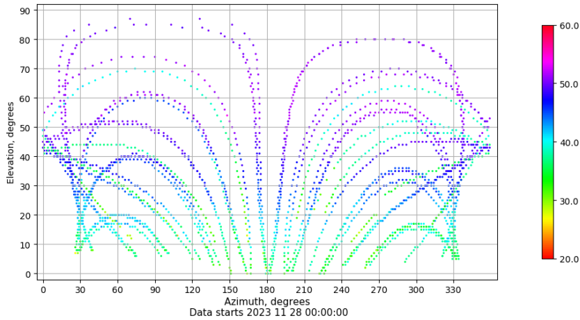
Azimuth-elevation plot for station LALA. Signal to Noise S1C Data file LALA00ESP_R_2023332.xtr
