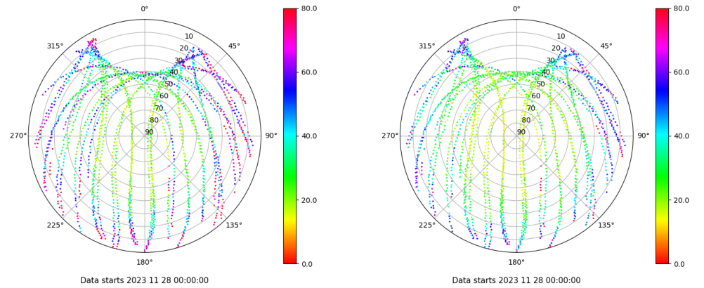
Skyplot for station LALA. Parameter M1C Data file LALA00ESP_R_2023332.xtr Skyplot for station LALA. Parameter M2C Data file LALA00ESP_R_2023332.xtr
