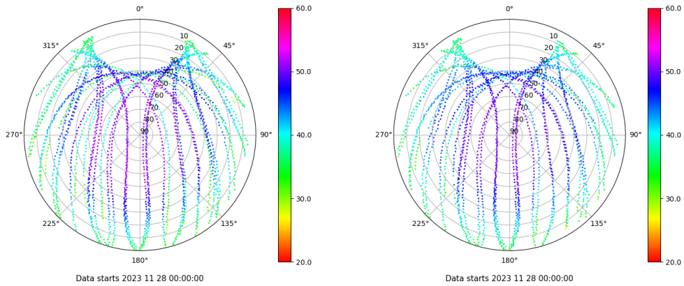
Skyplot for station LALA. Signal to Noise S1C Data file LALA00ESP_R_2023332.xtr Skyplot for station LALA. Signal to Noise S2C Data file LALA00ESP_R_2023332.xtr
