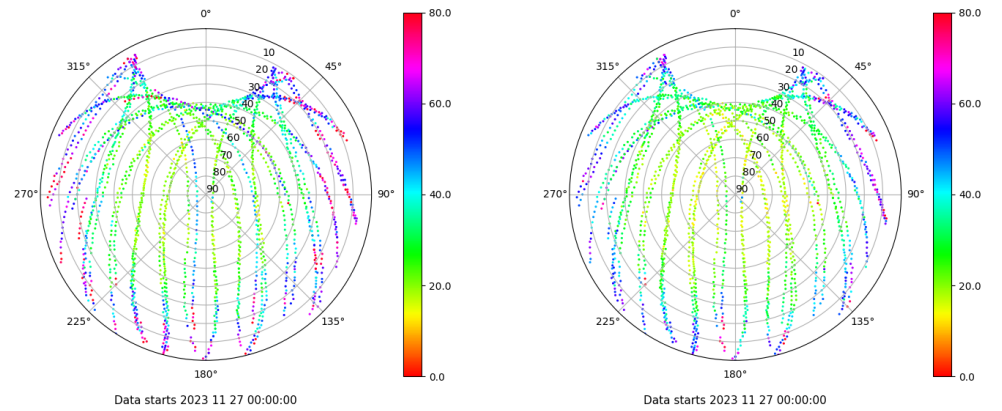
Skyplot for station LALA. Parameter M1C Data file LALA00ESP_R_2023331.xtr Skyplot for station LALA. Parameter M2C Data file LALA00ESP_R_2023331.xtr
