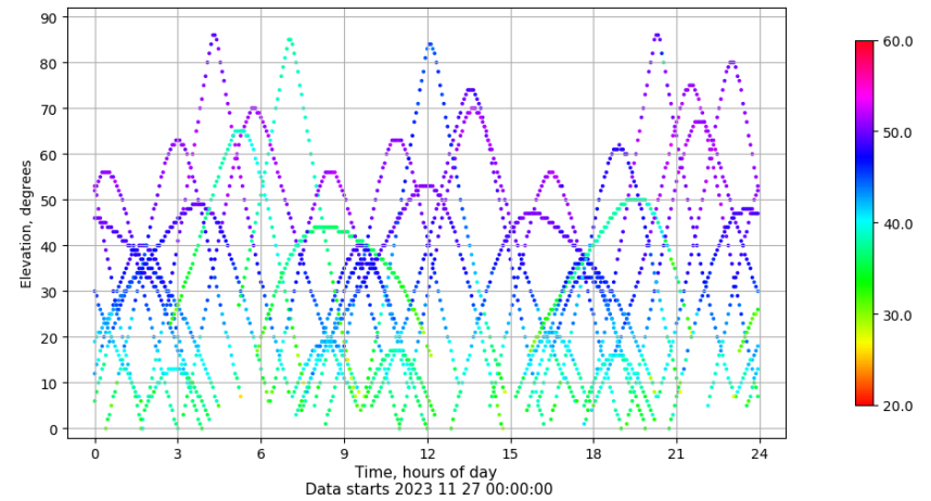
Time-elevation plot for station LALA. Signal to Noise S1C Data file LALA00ESP_R_2023331.xtr
