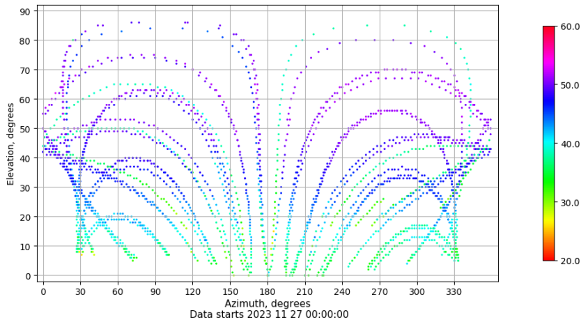
Azimuth-elevation plot for station LALA. Signal to Noise S1C Data file LALA00ESP_R_2023331.xtr
