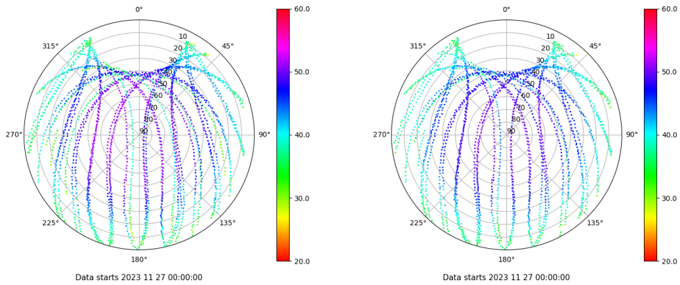
Skyplot for station LALA. Signal to Noise S1C Data file LALA00ESP_R_2023331.xtr Skyplot for station LALA. Signal to Noise S2C Data file LALA00ESP_R_2023331.xtr
