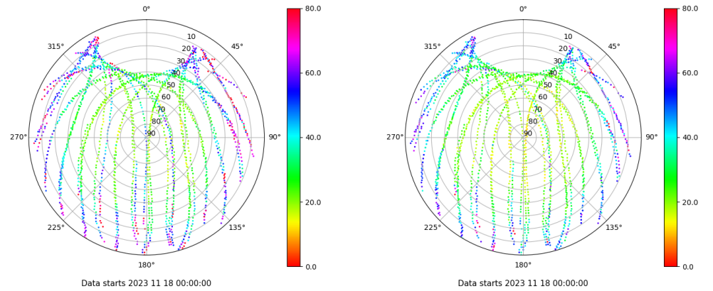
Skyplot for station LALA. Parameter M1C Data file LALA00ESP_R_2023322.xtr Skyplot for station LALA. Parameter M2C Data file LALA00ESP_R_2023322.xtr
