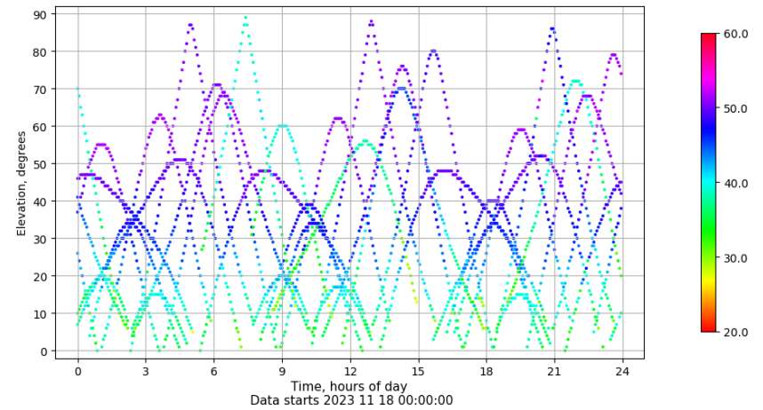
Time-elevation plot for station LALA. Signal to Noise S1C Data file LALA00ESP_R_2023322.xtr
