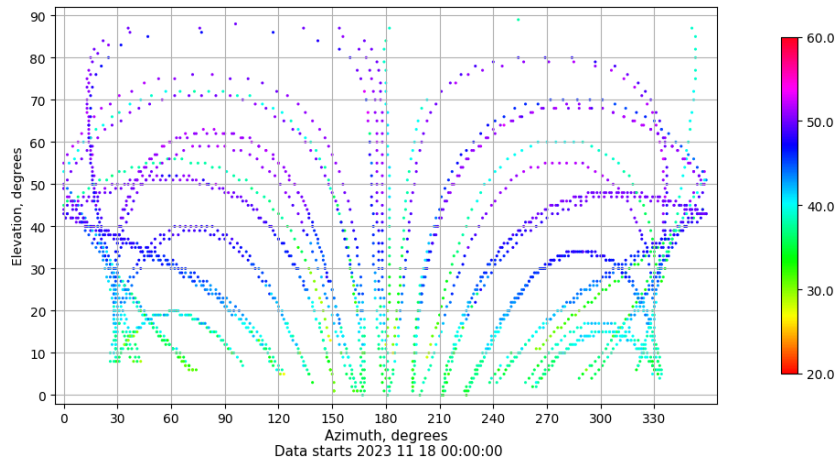
Azimuth-elevation plot for station LALA. Signal to Noise S1C Data file LALA00ESP_R_2023322.xtr
