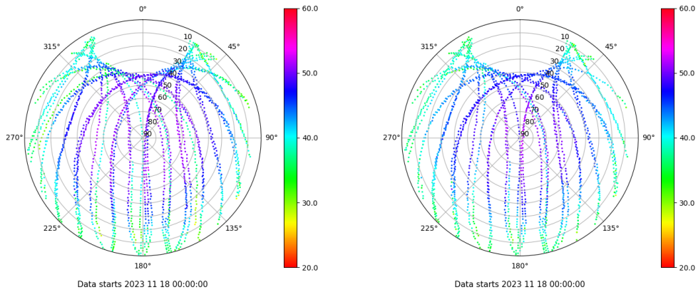
Skyplot for station LALA. Signal to Noise S1C Data file LALA00ESP_R_2023322.xtr Skyplot for station LALA. Signal to Noise S2C Data file LALA00ESP_R_2023322.xtr
