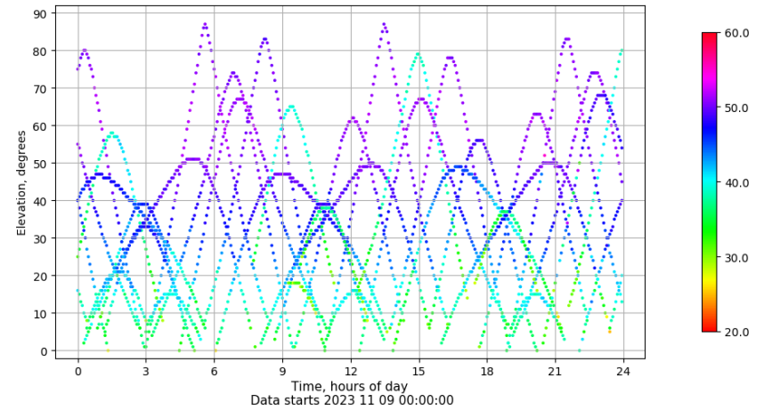
Time-elevation plot for station LALA. Signal to Noise S1C Data file LALA00ESP_R_2023313.xtr
