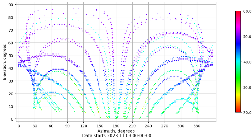
Azimuth-elevation plot for station LALA. Signal to Noise S1C Data file LALA00ESP_R_2023313.xtr
