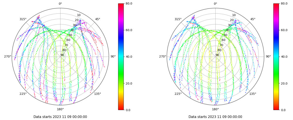
Skyplot for station LALA. Parameter M1C Data file LALA00ESP_R_2023313.xtr Skyplot for station LALA. Parameter M2C Data file LALA00ESP_R_2023313.xtr
