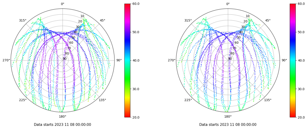
Skyplot for station LALA. Signal to Noise S1C Data file LALA00ESP_R_2023312.xtr Skyplot for station LALA. Signal to Noise S2C Data file LALA00ESP_R_2023312.xtr
