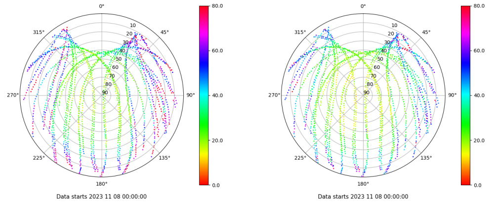
Skyplot for station LALA. Parameter M1C Data file LALA00ESP_R_2023312.xtr Skyplot for station LALA. Parameter M2C Data file LALA00ESP_R_2023312.xtr
