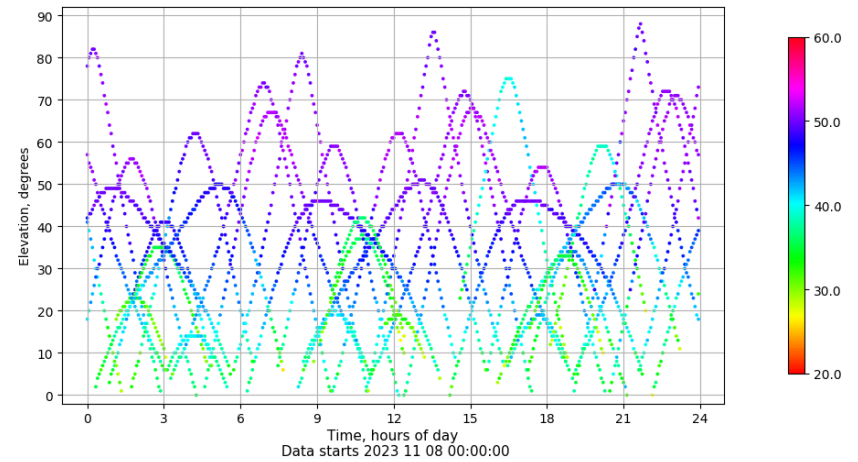
Time-elevation plot for station LALA. Signal to Noise S1C Data file LALA00ESP_R_2023312.xtr
