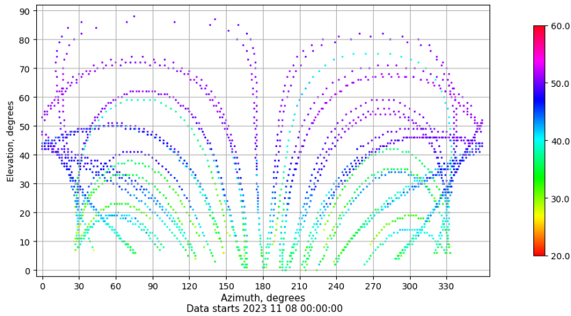
Azimuth-elevation plot for station LALA. Signal to Noise S1C Data file LALA00ESP_R_2023312.xtr
