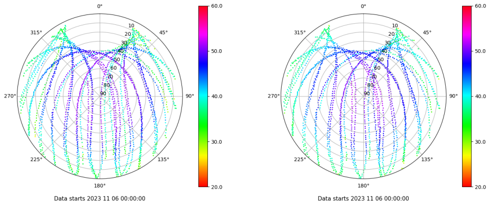
Skyplot for station LALA. Signal to Noise S1C Data file LALA00ESP_R_2023310.xtr Skyplot for station LALA. Signal to Noise S2C Data file LALA00ESP_R_2023310.xtr
