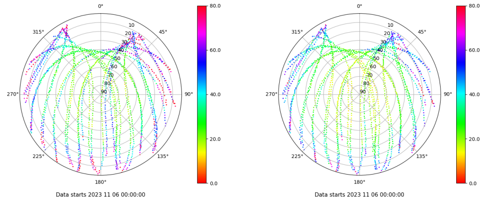
Skyplot for station LALA. Parameter M1C Data file LALA00ESP_R_2023310.xtr Skyplot for station LALA. Parameter M2C Data file LALA00ESP_R_2023310.xtr
