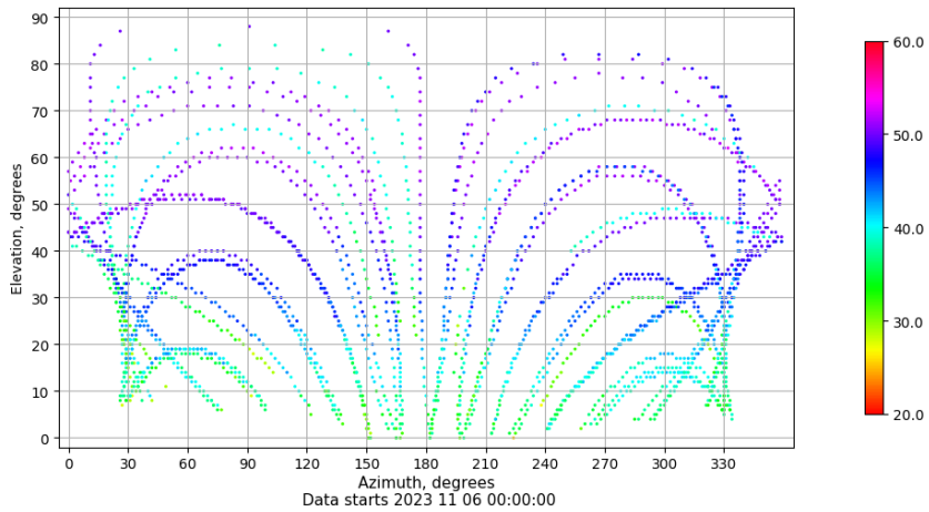
Azimuth-elevation plot for station LALA. Signal to Noise S1C Data file LALA00ESP_R_2023310.xtr
