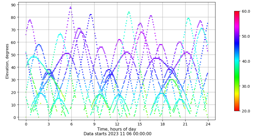
Time-elevation plot for station LALA. Signal to Noise S1C Data file LALA00ESP_R_2023310.xtr
