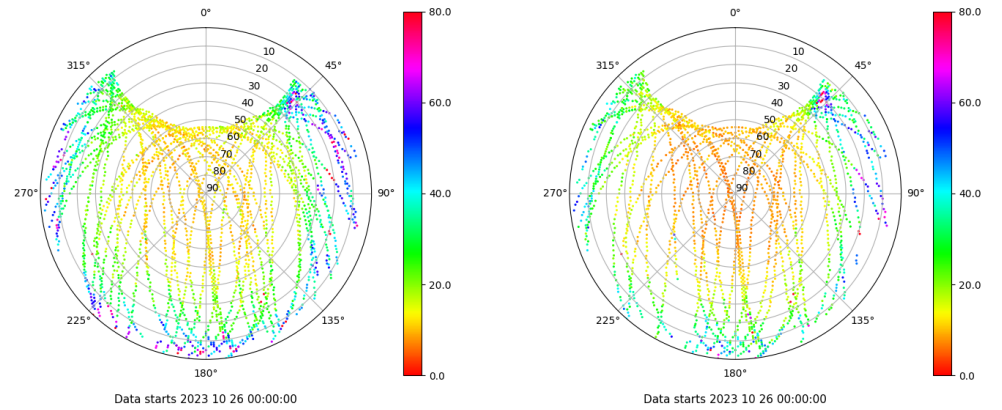
Skyplot for station LALA. Parameter M1C Data file LALA00ESP_R_2023299.xtr Skyplot for station LALA. Parameter M2X Data file LALA00ESP_R_2023299.xtr
