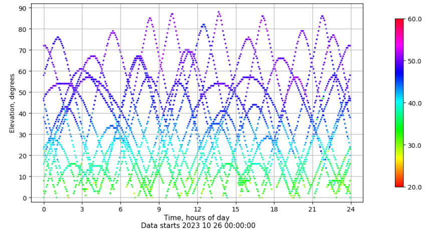
Time-elevation plot for station LALA. Signal to Noise S1C Data file LALA00ESP_R_2023299.xtr
