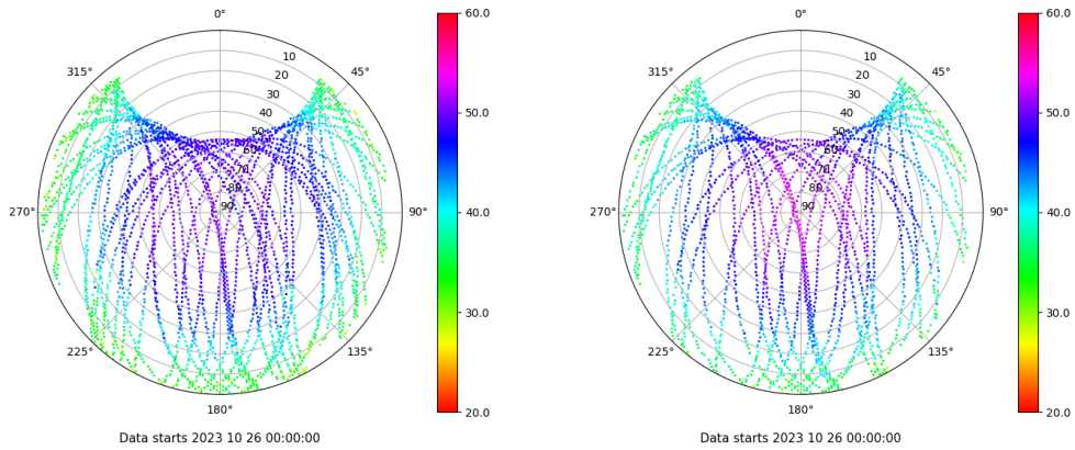
Skyplot for station LALA. Signal to Noise S1C Data file LALA00ESP_R_2023299.xtr Skyplot for station LALA. Signal to Noise S2X Data file LALA00ESP_R_2023299.xtr
