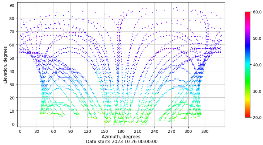
Azimuth-elevation plot for station LALA. Signal to Noise S1C Data file LALA00ESP_R_2023299.xtr
