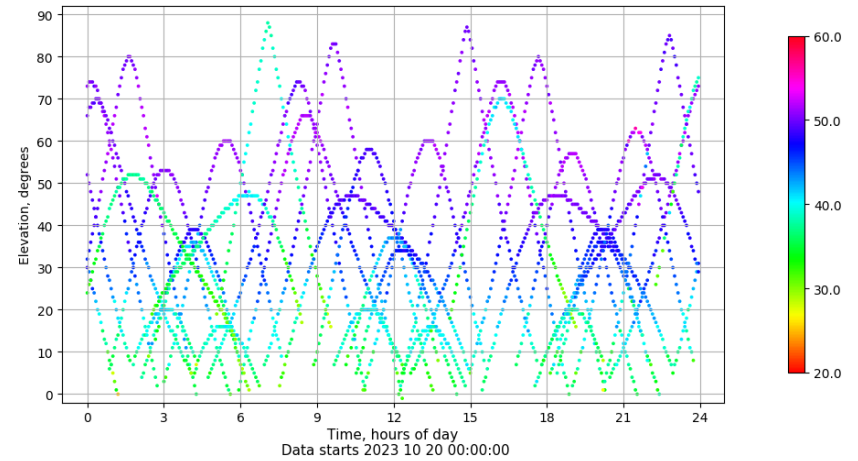
Time-elevation plot for station LALA. Signal to Noise S1C Data file LALA00ESP_R_2023293.xtr
