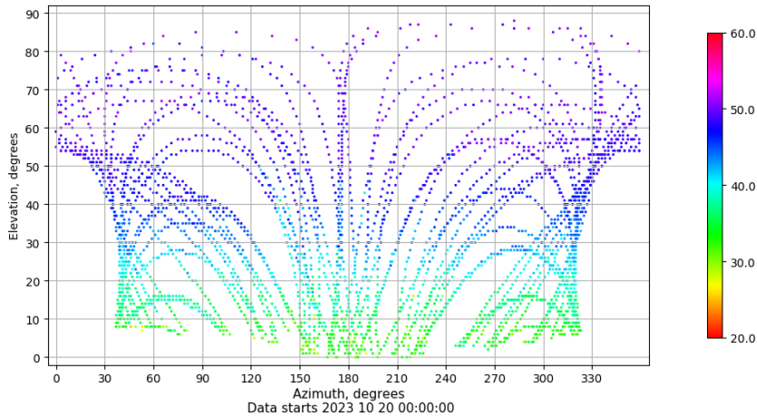
Azimuth-elevation plot for station LALA. Signal to Noise S1C Data file LALA00ESP_R_2023293.xtr
