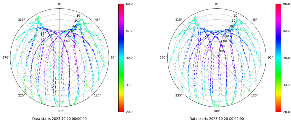
Skyplot for station LALA. Signal to Noise S1C Data file LALA00ESP_R_2023293.xtr Skyplot for station LALA. Signal to Noise S2C Data file LALA00ESP_R_2023293.xtr
