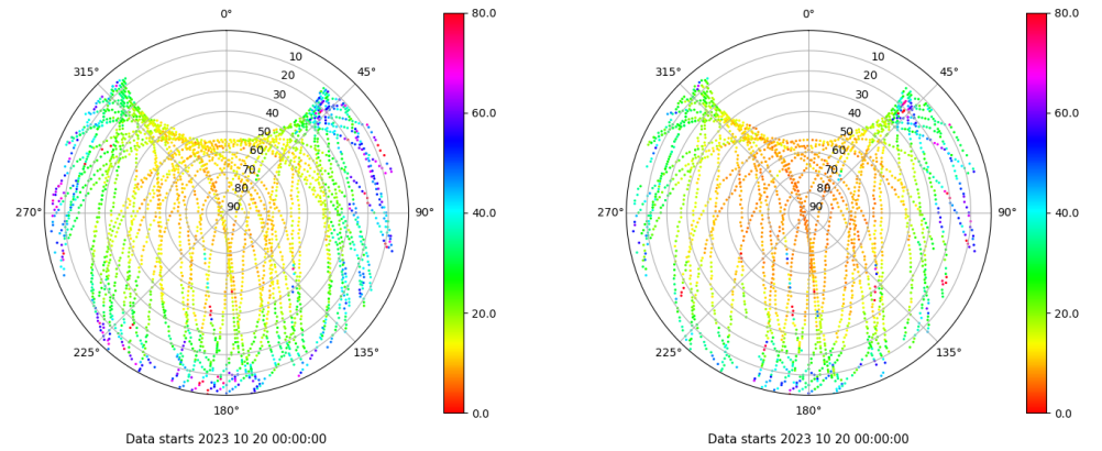
Skyplot for station LALA. Parameter M1C Data file LALA00ESP_R_2023293.xtr Skyplot for station LALA. Parameter M2X Data file LALA00ESP_R_2023293.xtr
