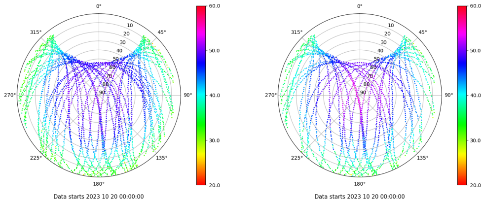
Skyplot for station LALA. Signal to Noise S1C Data file LALA00ESP_R_2023293.xtr Skyplot for station LALA. Signal to Noise S2X Data file LALA00ESP_R_2023293.xtr
