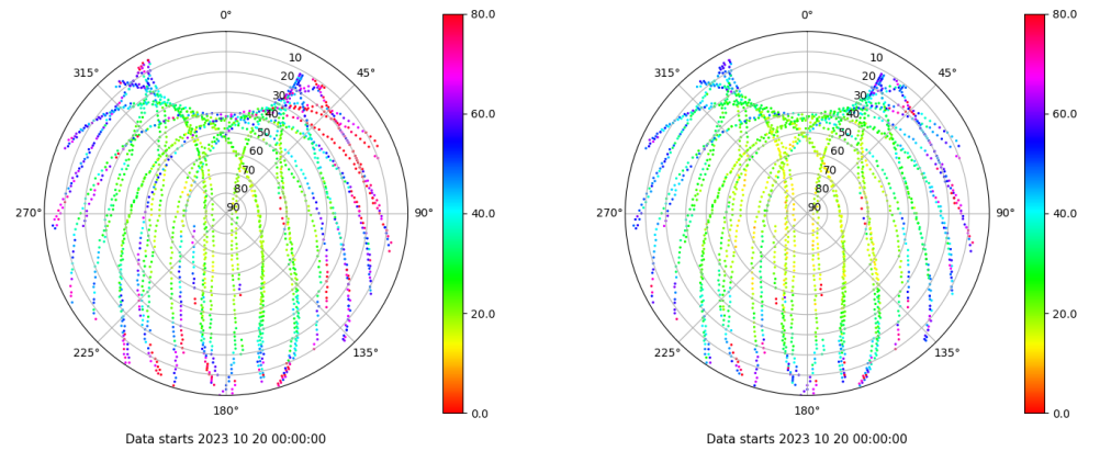
Skyplot for station LALA. Parameter M1C Data file LALA00ESP_R_2023293.xtr Skyplot for station LALA. Parameter M2C Data file LALA00ESP_R_2023293.xtr
