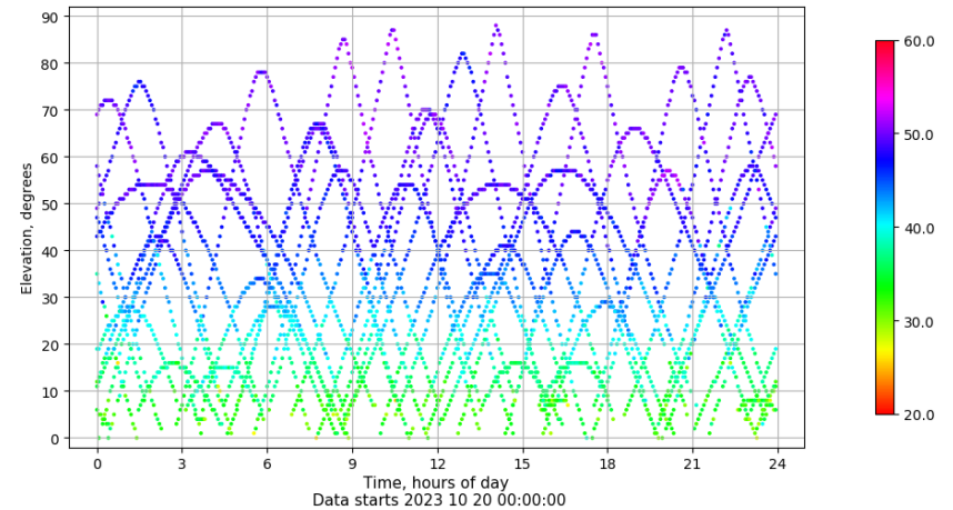
Time-elevation plot for station LALA. Signal to Noise S1C Data file LALA00ESP_R_2023293.xtr
