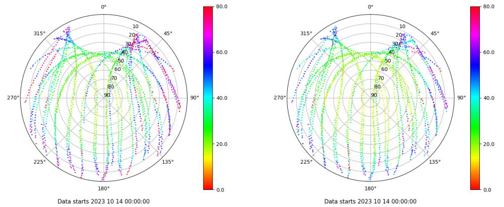
Skyplot for station LALA. Parameter M1C Data file LALA00ESP_R_2023287.xtr Skyplot for station LALA. Parameter M2C Data file LALA00ESP_R_2023287.xtr
