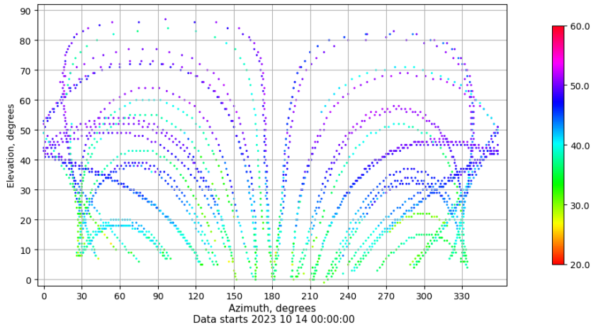
Azimuth-elevation plot for station LALA. Signal to Noise S1C Data file LALA00ESP_R_2023287.xtr
