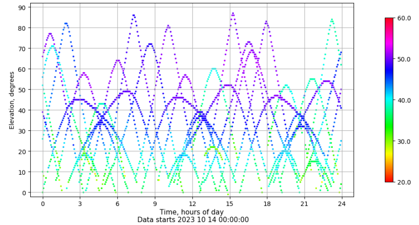
Time-elevation plot for station LALA. Signal to Noise S1C Data file LALA00ESP_R_2023287.xtr
