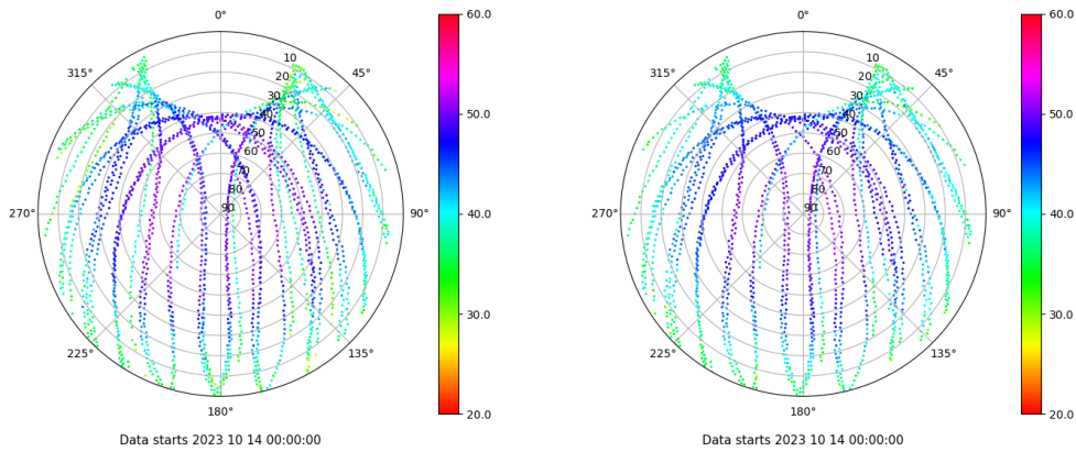
Skyplot for station LALA. Signal to Noise S1C Data file LALA00ESP_R_2023287.xtr Skyplot for station LALA. Signal to Noise S2C Data file LALA00ESP_R_2023287.xtr
