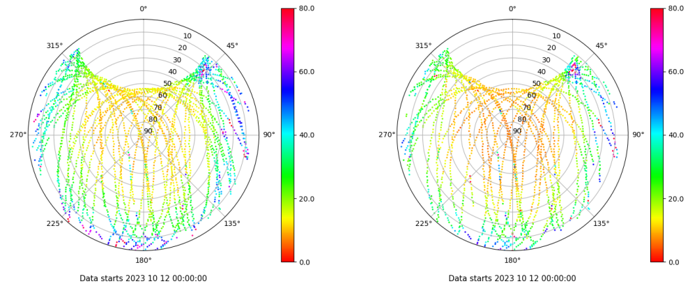
Skyplot for station LALA. Parameter M1C Data file LALA00ESP_R_2023285.xtr Skyplot for station LALA. Parameter M2X Data file LALA00ESP_R_2023285.xtr
