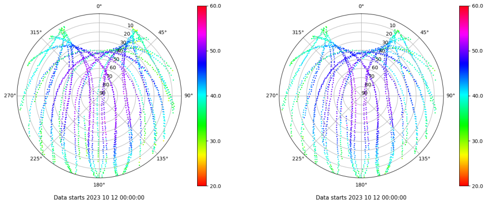
Skyplot for station LALA. Signal to Noise S1C Data file LALA00ESP_R_2023285.xtr Skyplot for station LALA. Signal to Noise S2C Data file LALA00ESP_R_2023285.xtr
