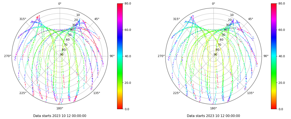
Skyplot for station LALA. Parameter M1C Data file LALA00ESP_R_2023285.xtr Skyplot for station LALA. Parameter M2C Data file LALA00ESP_R_2023285.xtr
