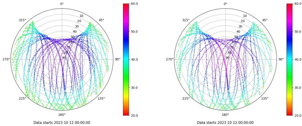
Skyplot for station LALA. Signal to Noise S1C Data file LALA00ESP_R_2023285.xtr Skyplot for station LALA. Signal to Noise S2X Data file LALA00ESP_R_2023285.xtr
