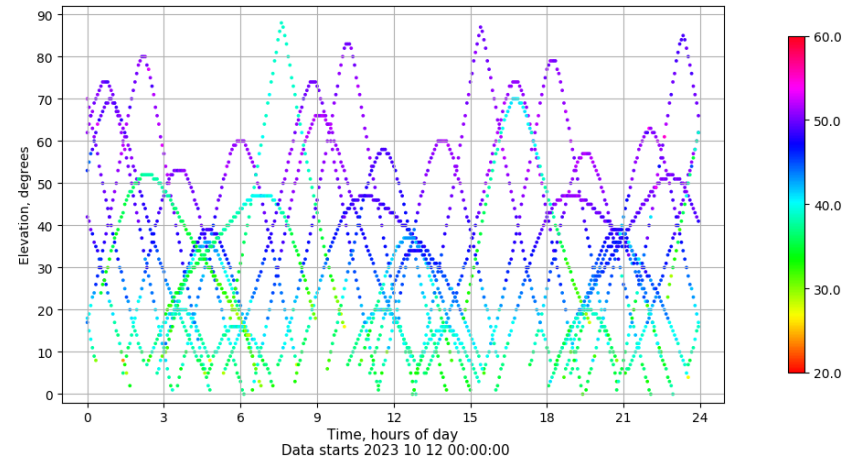
Time-elevation plot for station LALA. Signal to Noise S1C Data file LALA00ESP_R_2023285.xtr
