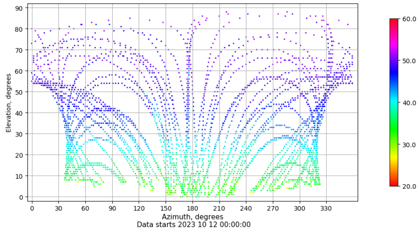
Azimuth-elevation plot for station LALA. Signal to Noise S1C Data file LALA00ESP_R_2023285.xtr
