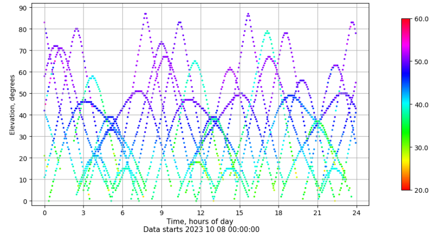
Time-elevation plot for station LALA. Signal to Noise S1C Data file LALA00ESP_R_2023281.xtr
