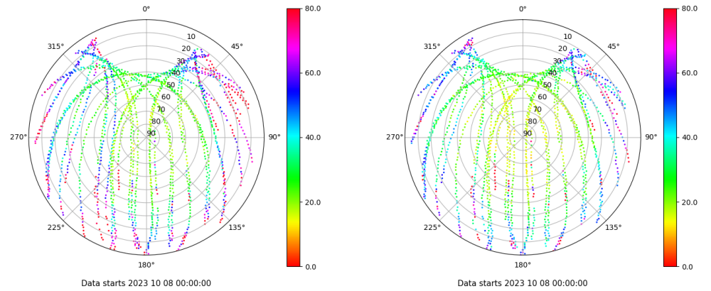
Skyplot for station LALA. Parameter M1C Data file LALA00ESP_R_2023281.xtr Skyplot for station LALA. Parameter M2C Data file LALA00ESP_R_2023281.xtr
