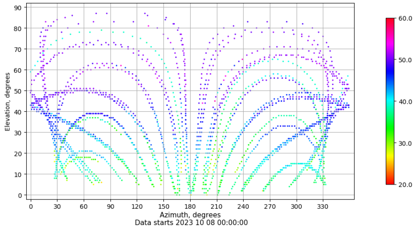
Azimuth-elevation plot for station LALA. Signal to Noise S1C Data file LALA00ESP_R_2023281.xtr
