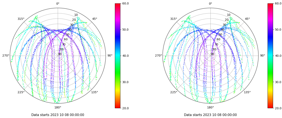
Skyplot for station LALA. Signal to Noise S1C Data file LALA00ESP_R_2023281.xtr Skyplot for station LALA. Signal to Noise S2C Data file LALA00ESP_R_2023281.xtr
