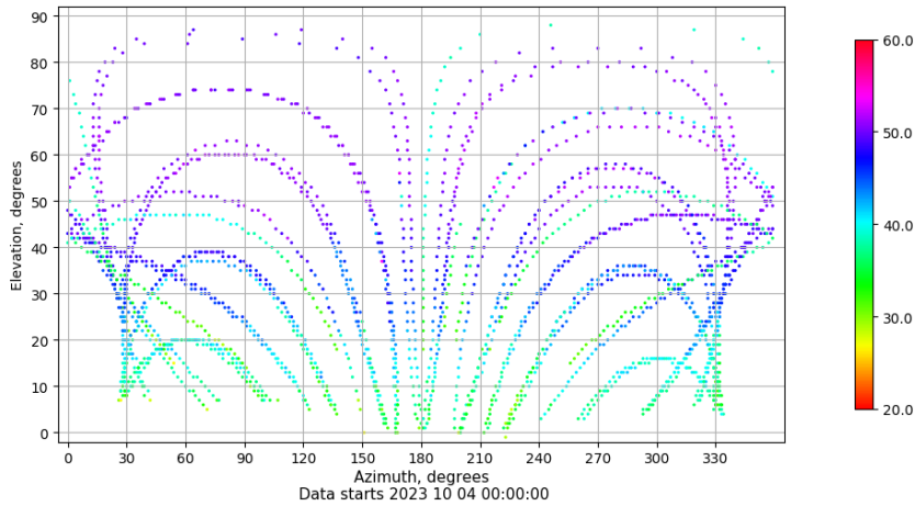
Azimuth-elevation plot for station LALA. Signal to Noise S1C Data file LALA00ESP_R_2023277.xtr
