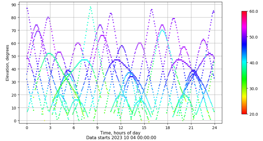
Time-elevation plot for station LALA. Signal to Noise S1C Data file LALA00ESP_R_2023277.xtr
