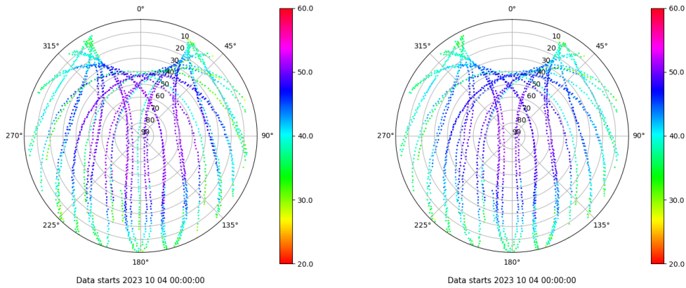
Skyplot for station LALA. Signal to Noise S1C Data file LALA00ESP_R_2023277.xtr Skyplot for station LALA. Signal to Noise S2C Data file LALA00ESP_R_2023277.xtr
