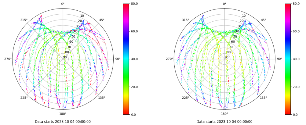
Skyplot for station LALA. Parameter M1C Data file LALA00ESP_R_2023277.xtr Skyplot for station LALA. Parameter M2C Data file LALA00ESP_R_2023277.xtr
