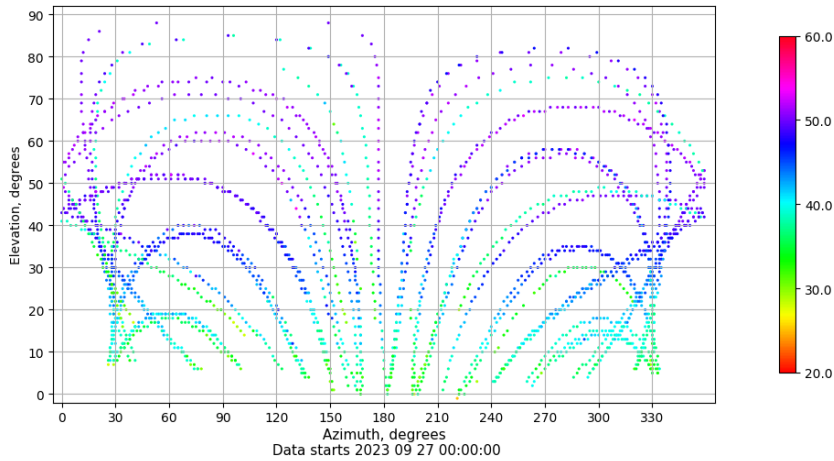
Azimuth-elevation plot for station LALA. Signal to Noise S1C Data file LALA00ESP_R_2023270.xtr
