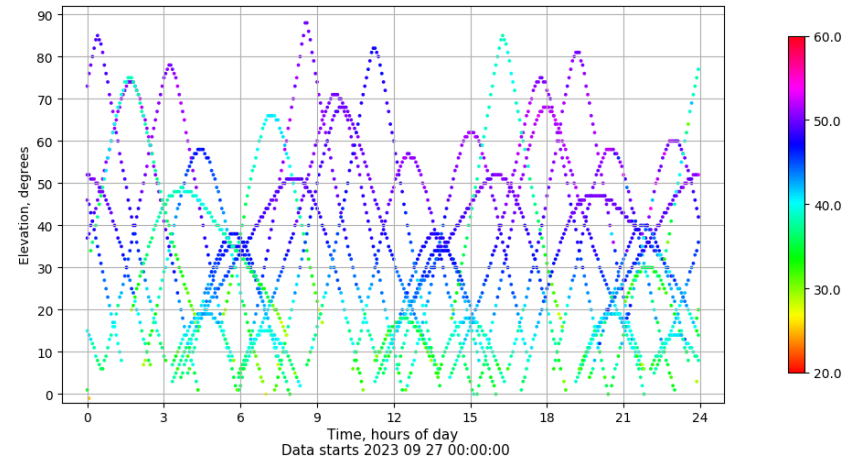
Time-elevation plot for station LALA. Signal to Noise S1C Data file LALA00ESP_R_2023270.xtr
