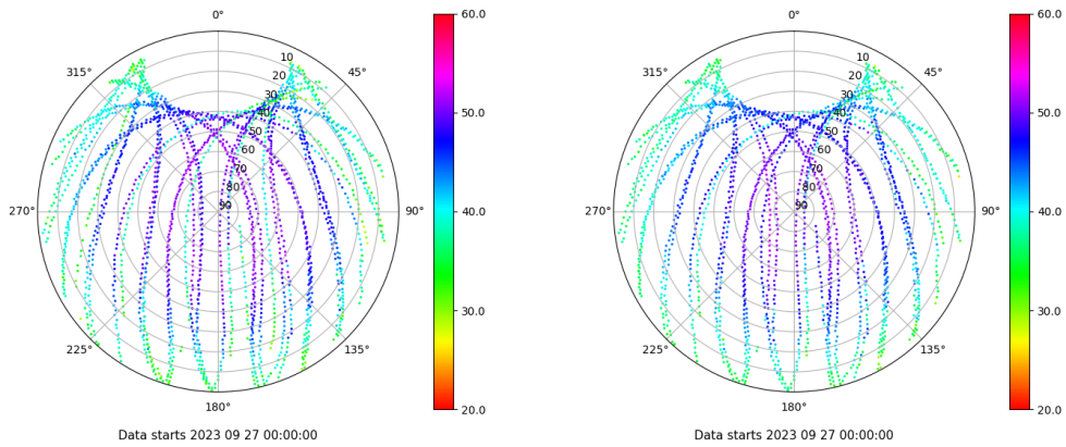
Skyplot for station LALA. Signal to Noise S1C Data file LALA00ESP_R_2023270.xtr Skyplot for station LALA. Signal to Noise S2C Data file LALA00ESP_R_2023270.xtr
