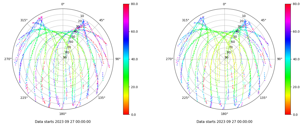
Skyplot for station LALA. Parameter M1C Data file LALA00ESP_R_2023270.xtr Skyplot for station LALA. Parameter M2C Data file LALA00ESP_R_2023270.xtr
