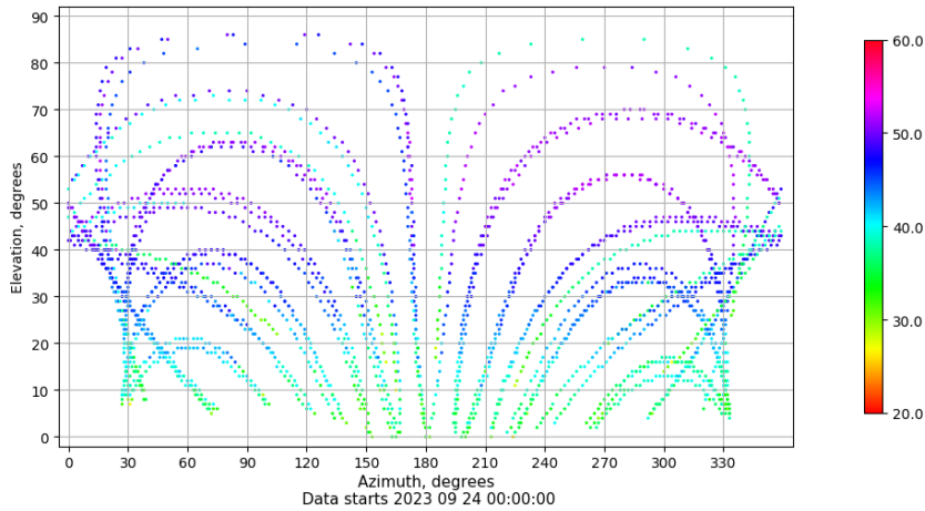
Azimuth-elevation plot for station LALA. Signal to Noise S1C Data file LALA00ESP_R_2023267.xtr
