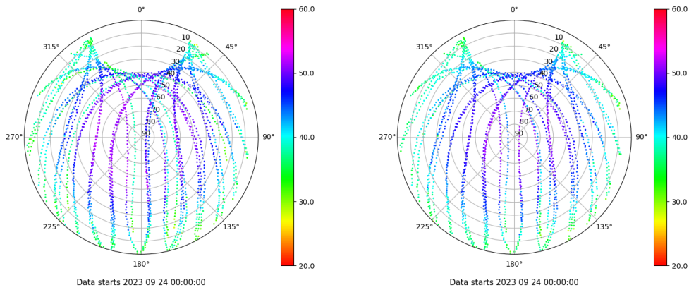
Skyplot for station LALA. Signal to Noise S1C Data file LALA00ESP_R_2023267.xtr Skyplot for station LALA. Signal to Noise S2C Data file LALA00ESP_R_2023267.xtr
