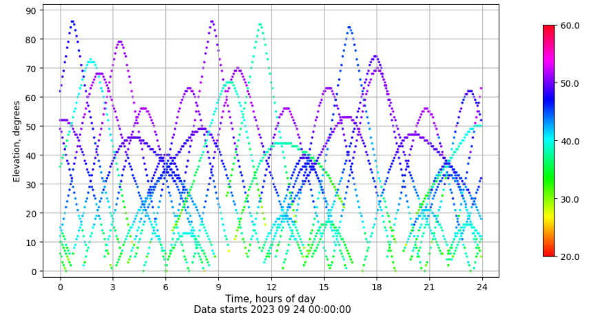
Time-elevation plot for station LALA. Signal to Noise S1C Data file LALA00ESP_R_2023267.xtr
