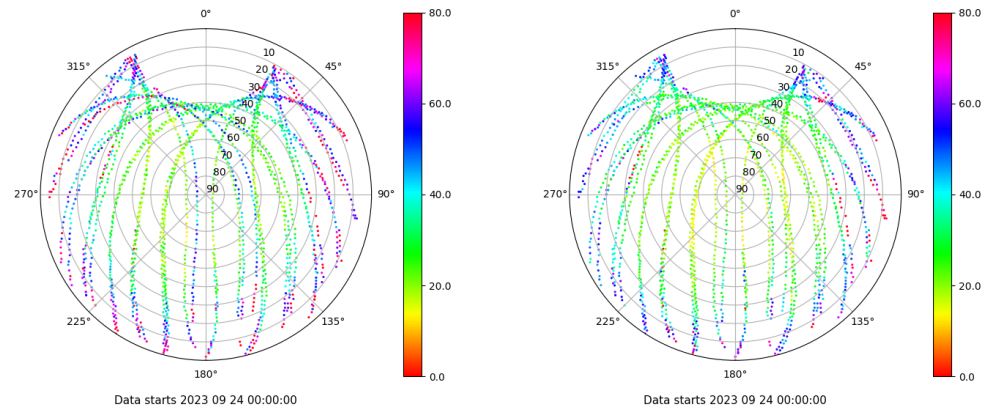
Skyplot for station LALA. Parameter M1C Data file LALA00ESP_R_2023267.xtr Skyplot for station LALA. Parameter M2C Data file LALA00ESP_R_2023267.xtr
