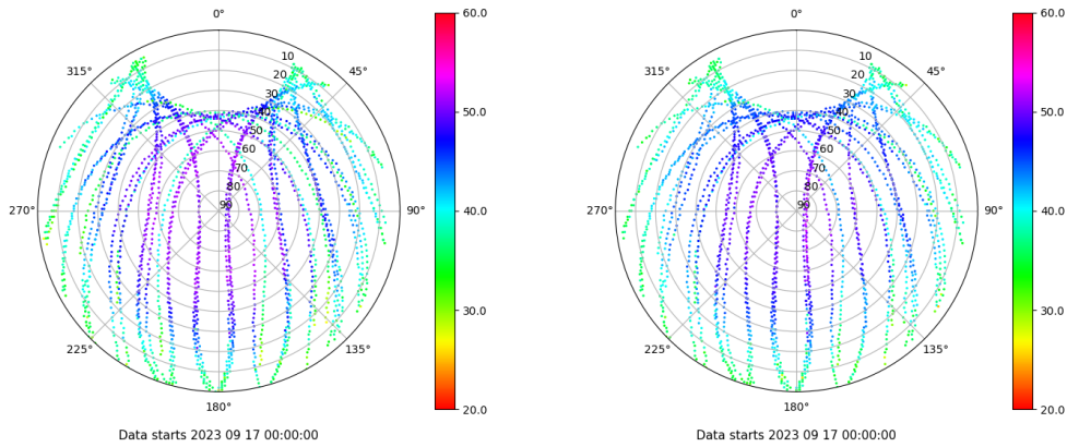
Skyplot for station LALA. Signal to Noise S1C Data file LALA00ESP_R_2023260.xtr Skyplot for station LALA. Signal to Noise S2C Data file LALA00ESP_R_2023260.xtr
