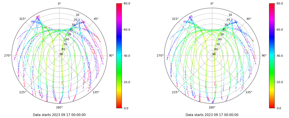
Skyplot for station LALA. Parameter M1C Data file LALA00ESP_R_2023260.xtr Skyplot for station LALA. Parameter M2C Data file LALA00ESP_R_2023260.xtr
