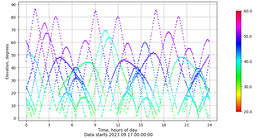
Time-elevation plot for station LALA. Signal to Noise S1C Data file LALA00ESP_R_2023260.xtr
