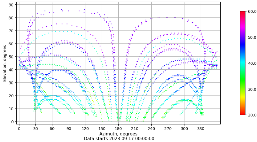
Azimuth-elevation plot for station LALA. Signal to Noise S1C Data file LALA00ESP_R_2023260.xtr
