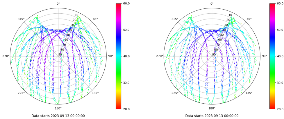
Skyplot for station LALA. Signal to Noise S1C Data file LALA00ESP_R_2023256.xtr Skyplot for station LALA. Signal to Noise S2C Data file LALA00ESP_R_2023256.xtr
