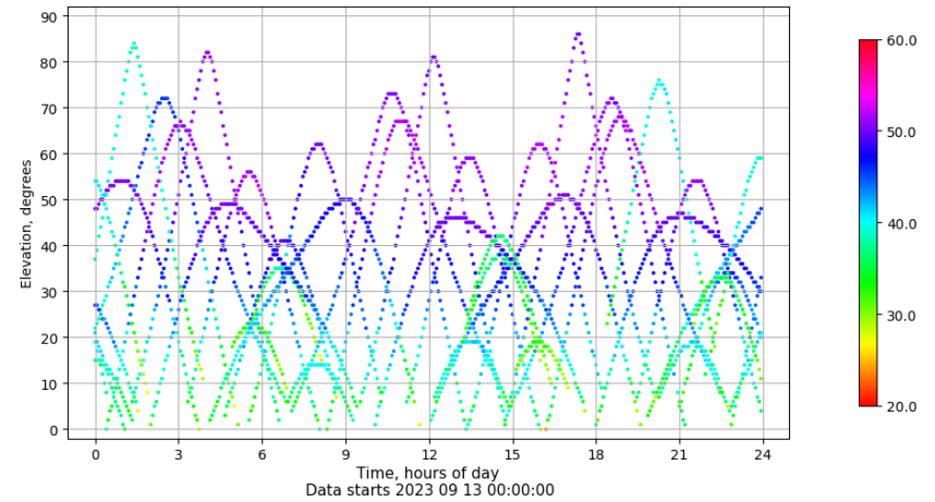
Time-elevation plot for station LALA. Signal to Noise S1C Data file LALA00ESP_R_2023256.xtr
