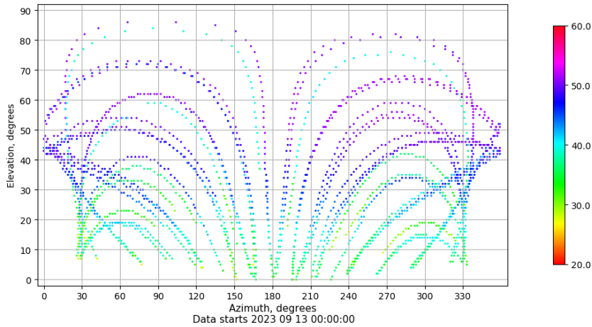
Azimuth-elevation plot for station LALA. Signal to Noise S1C Data file LALA00ESP_R_2023256.xtr
