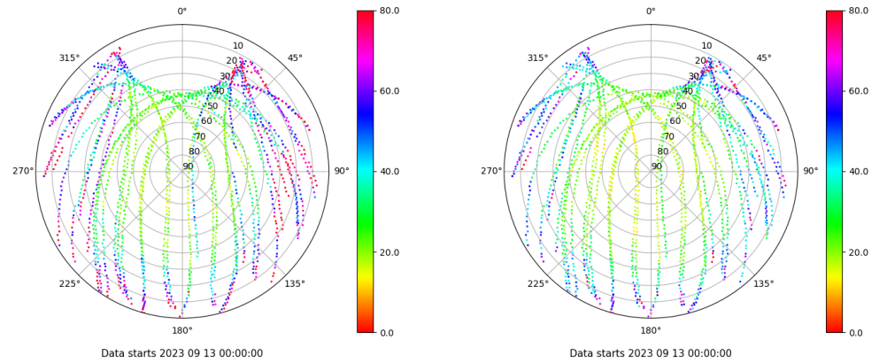
Skyplot for station LALA. Parameter M1C Data file LALA00ESP_R_2023256.xtr Skyplot for station LALA. Parameter M2C Data file LALA00ESP_R_2023256.xtr
