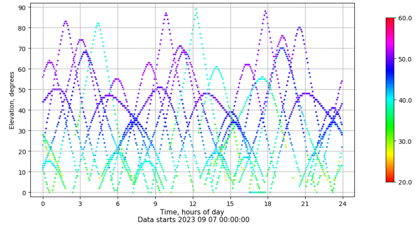
Time-elevation plot for station LALA. Signal to Noise S1C Data file LALA00ESP_R_2023250.xtr
