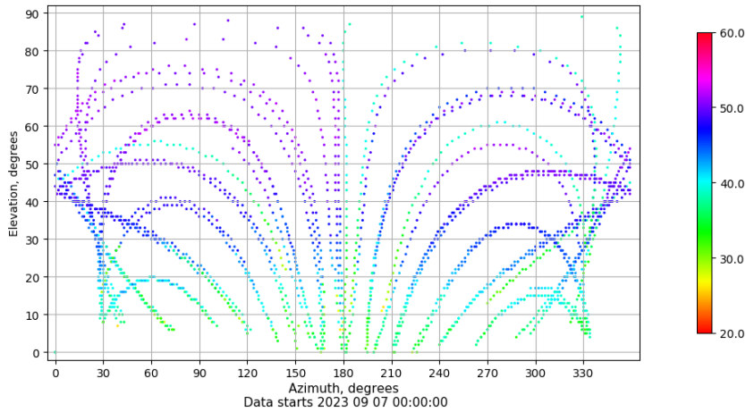
Azimuth-elevation plot for station LALA. Signal to Noise S1C Data file LALA00ESP_R_2023250.xtr
