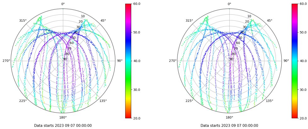
Skyplot for station LALA. Signal to Noise S1C Data file LALA00ESP_R_2023250.xtr Skyplot for station LALA. Signal to Noise S2C Data file LALA00ESP_R_2023250.xtr
