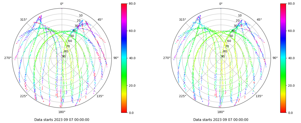
Skyplot for station LALA. Parameter M1C Data file LALA00ESP_R_2023250.xtr Skyplot for station LALA. Parameter M2C Data file LALA00ESP_R_2023250.xtr
