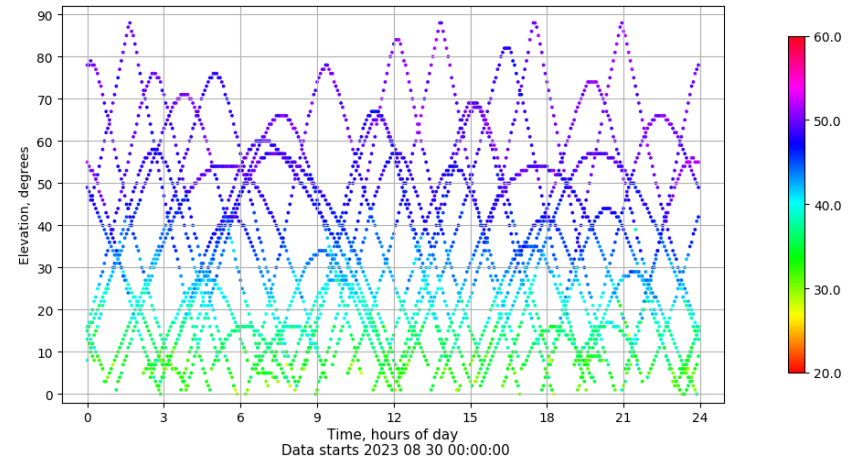
Time-elevation plot for station LALA. Signal to Noise S1C Data file LALA00ESP_R_2023242.xtr
