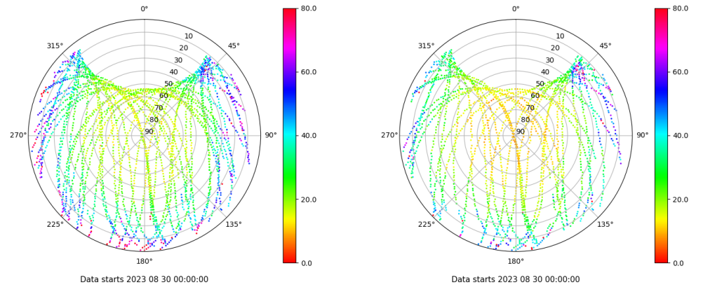
Skyplot for station LALA. Parameter M1C Data file LALA00ESP_R_2023242.xtr Skyplot for station LALA. Parameter M2X Data file LALA00ESP_R_2023242.xtr
