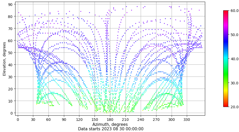
Azimuth-elevation plot for station LALA. Signal to Noise S1C Data file LALA00ESP_R_2023242.xtr
