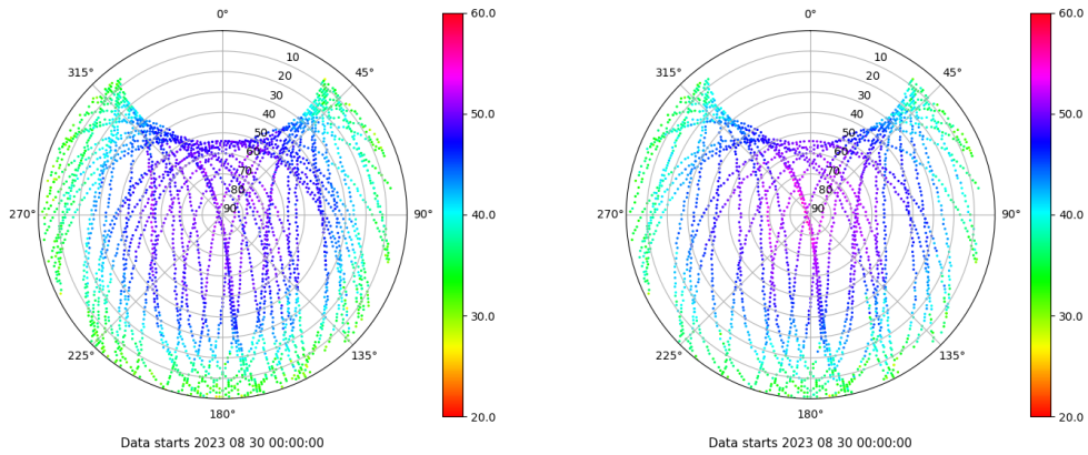
Skyplot for station LALA. Signal to Noise S1C Data file LALA00ESP_R_2023242.xtr Skyplot for station LALA. Signal to Noise S2X Data file LALA00ESP_R_2023242.xtr
