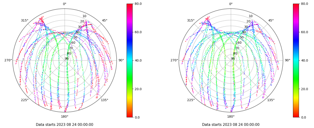
Skyplot for station LALA. Parameter M1C Data file LALA00ESP_R_2023236.xtr Skyplot for station LALA. Parameter M2C Data file LALA00ESP_R_2023236.xtr
