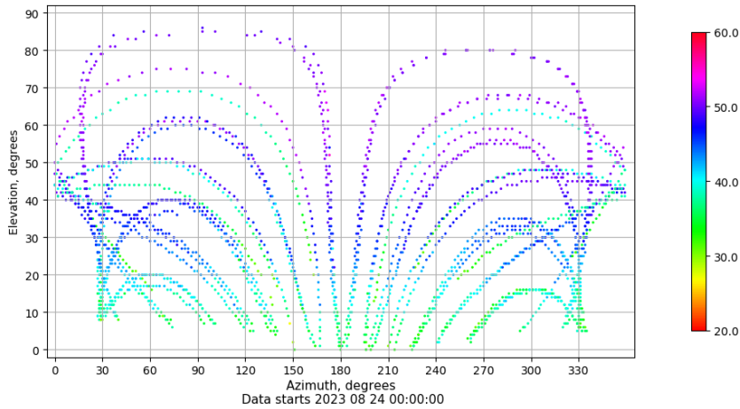
Azimuth-elevation plot for station LALA. Signal to Noise S1C Data file LALA00ESP_R_2023236.xtr
