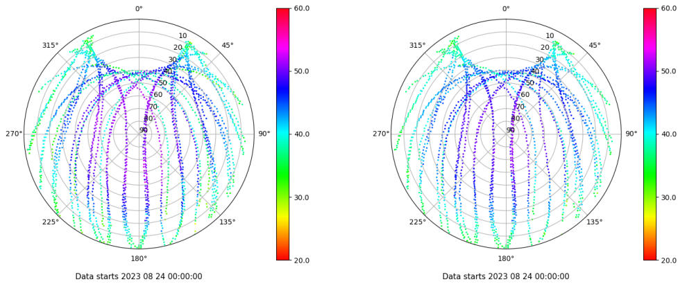
Skyplot for station LALA. Signal to Noise S1C Data file LALA00ESP_R_2023236.xtr Skyplot for station LALA. Signal to Noise S2C Data file LALA00ESP_R_2023236.xtr
