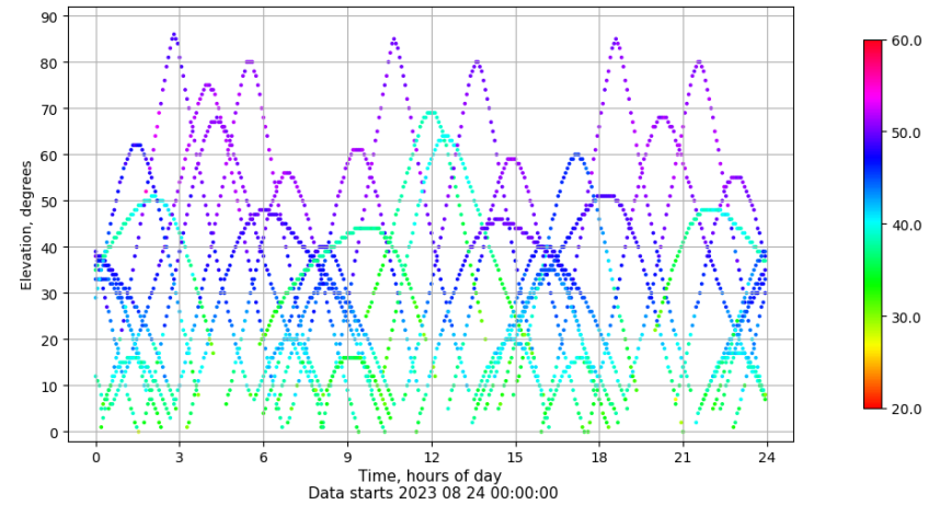
Time-elevation plot for station LALA. Signal to Noise S1C Data file LALA00ESP_R_2023236.xtr
