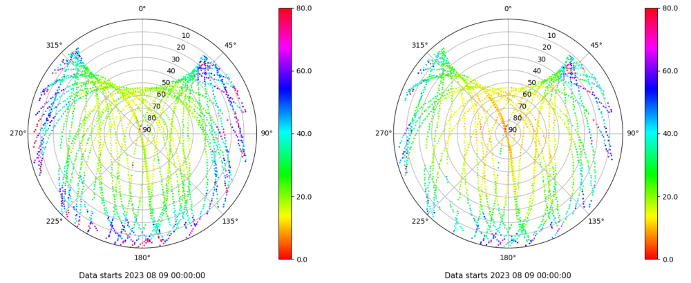
Skyplot for station LALA. Parameter M1C Data file LALA00ESP_R_2023221.xtr Skyplot for station LALA. Parameter M2X Data file LALA00ESP_R_2023221.xtr
