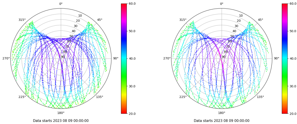
Skyplot for station LALA. Signal to Noise S1C Data file LALA00ESP_R_2023221.xtr Skyplot for station LALA. Signal to Noise S2X Data file LALA00ESP_R_2023221.xtr
