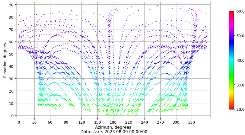
Azimuth-elevation plot for station LALA. Signal to Noise S1C Data file LALA00ESP_R_2023221.xtr
