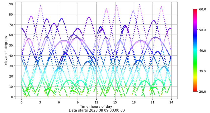
Time-elevation plot for station LALA. Signal to Noise S1C Data file LALA00ESP_R_2023221.xtr
