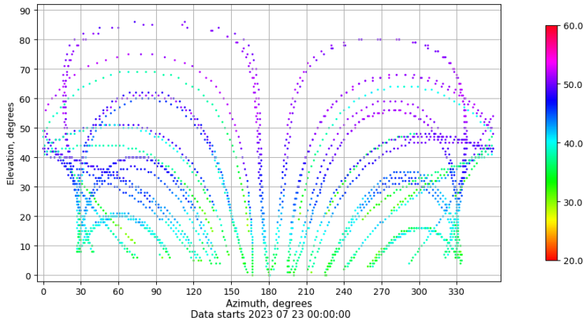
Azimuth-elevation plot for station LALA. Signal to Noise S1C Data file LALA00ESP_R_2023204.xtr
