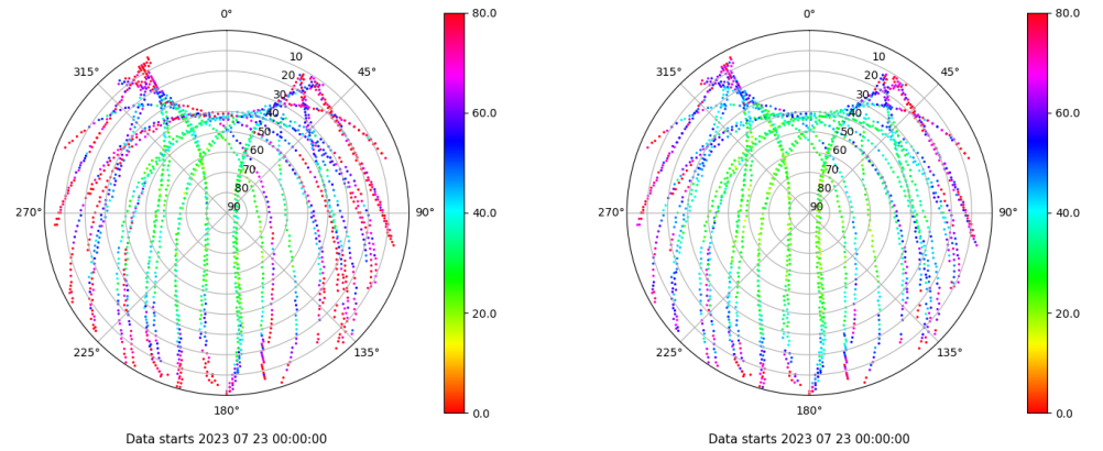
Skyplot for station LALA. Parameter M1C Data file LALA00ESP_R_2023204.xtr Skyplot for station LALA. Parameter M2C Data file LALA00ESP_R_2023204.xtr
