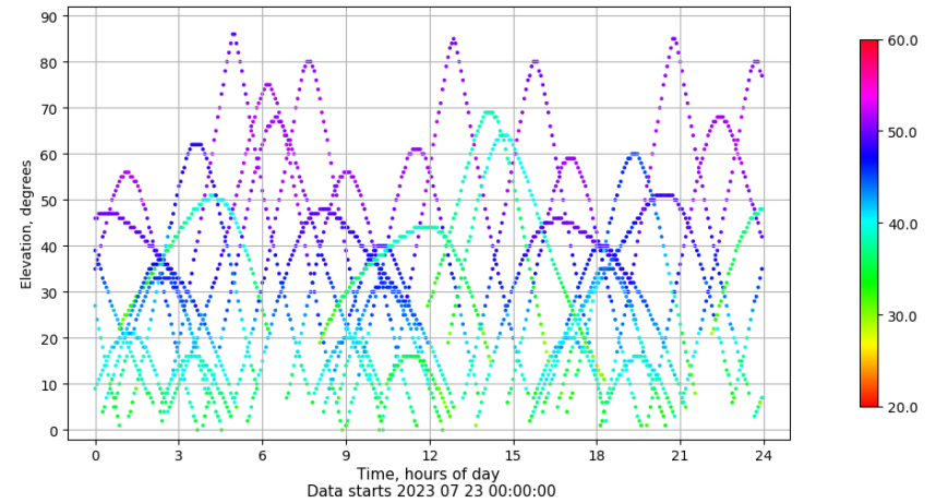
Time-elevation plot for station LALA. Signal to Noise S1C Data file LALA00ESP_R_2023204.xtr
