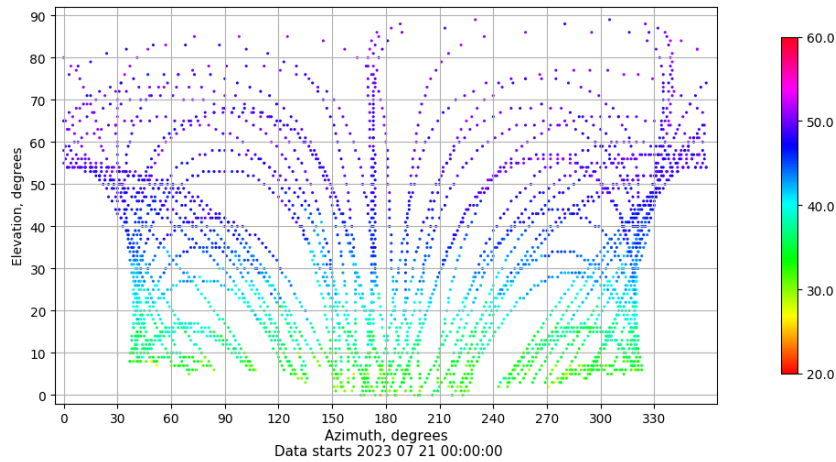
Azimuth-elevation plot for station LALA. Signal to Noise S1C Data file LALA00ESP_R_2023202.xtr
