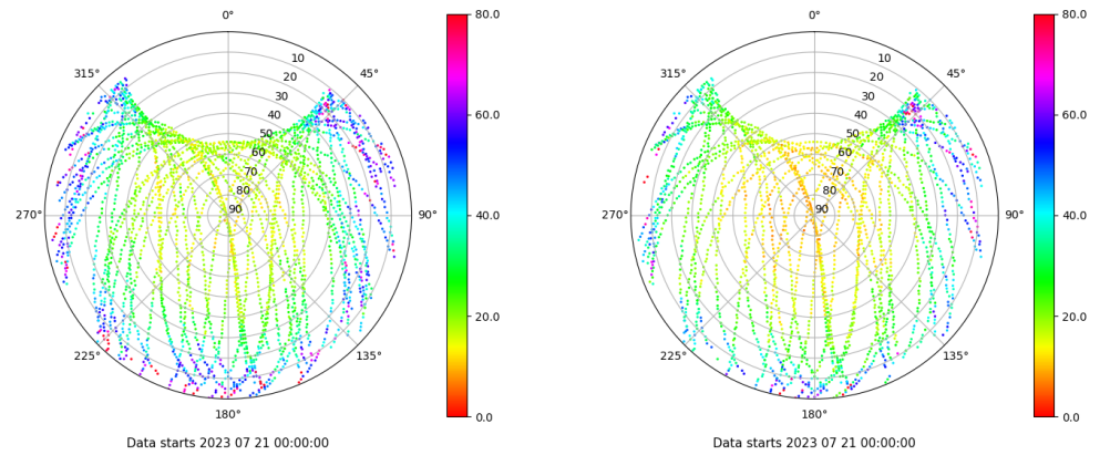
Skyplot for station LALA. Parameter M1C Data file LALA00ESP_R_2023202.xtr Skyplot for station LALA. Parameter M2X Data file LALA00ESP_R_2023202.xtr
