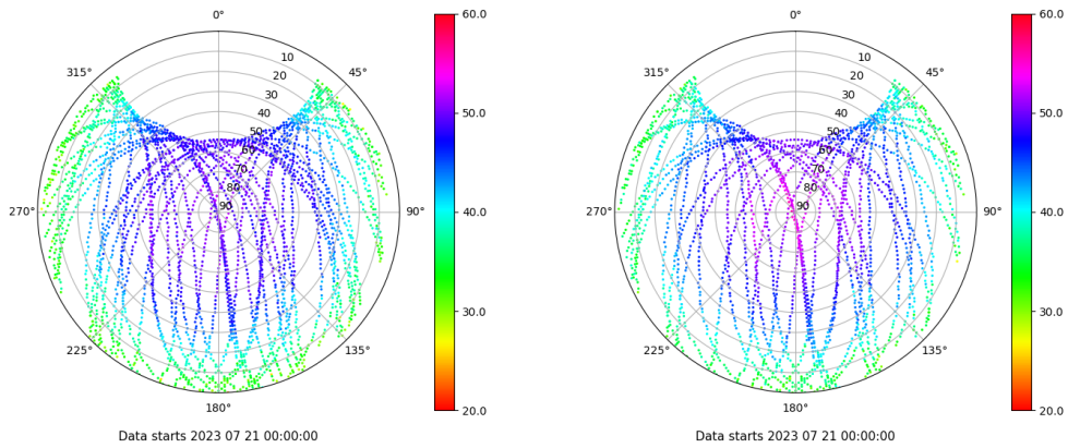
Skyplot for station LALA. Signal to Noise S1C Data file LALA00ESP_R_2023202.xtr Skyplot for station LALA. Signal to Noise S2X Data file LALA00ESP_R_2023202.xtr
