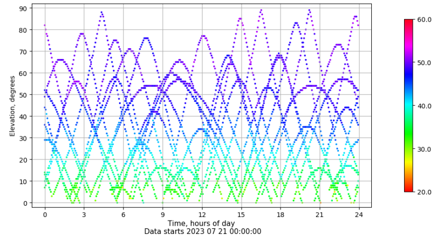
Time-elevation plot for station LALA. Signal to Noise S1C Data file LALA00ESP_R_2023202.xtr
