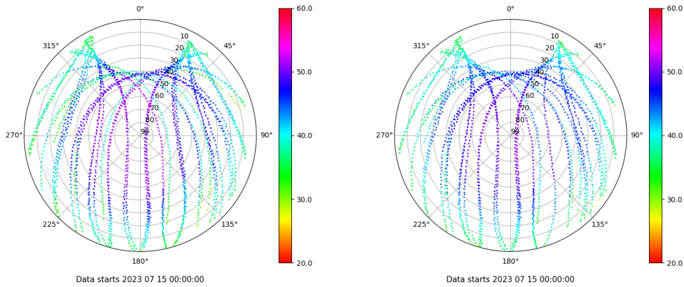
Skyplot for station LALA. Signal to Noise S1C Data file LALA00ESP_R_2023196.xtr Skyplot for station LALA. Signal to Noise S2C Data file LALA00ESP_R_2023196.xtr
