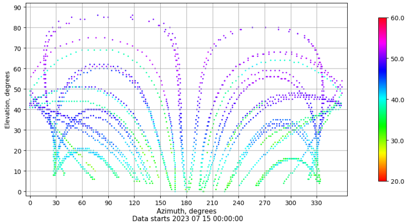
Azimuth-elevation plot for station LALA. Signal to Noise S1C Data file LALA00ESP_R_2023196.xtr
