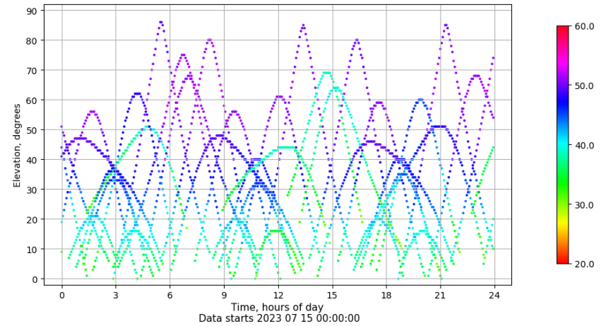
Time-elevation plot for station LALA. Signal to Noise S1C Data file LALA00ESP_R_2023196.xtr
