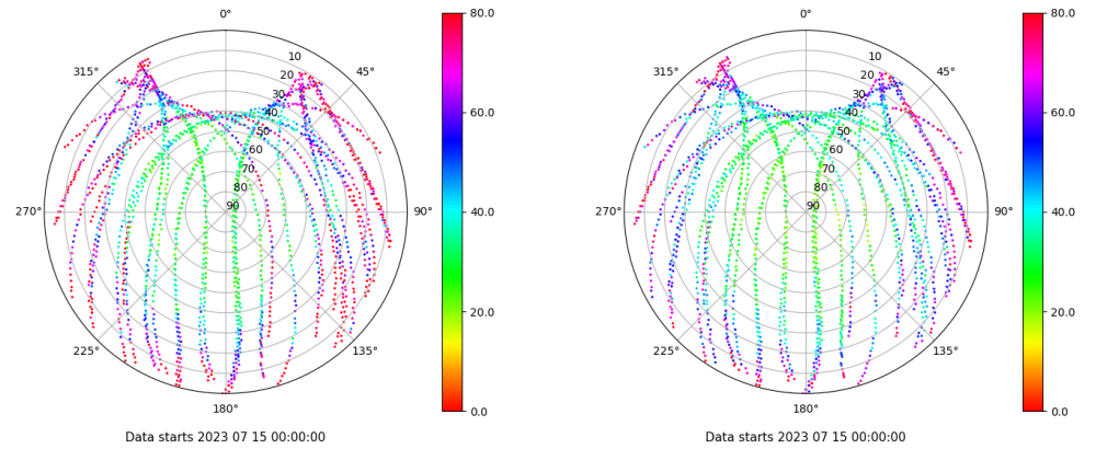
Skyplot for station LALA. Parameter M1C Data file LALA00ESP_R_2023196.xtr Skyplot for station LALA. Parameter M2C Data file LALA00ESP_R_2023196.xtr
