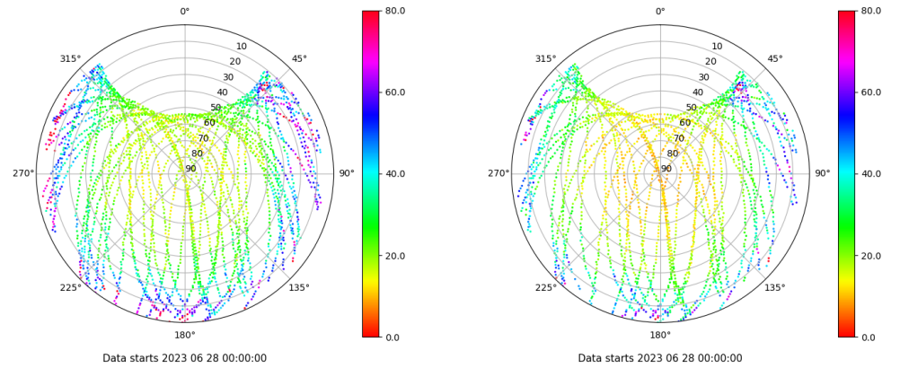
Skyplot for station LALA. Parameter M1C Data file LALA00ESP_R_2023179.xtr Skyplot for station LALA. Parameter M2X Data file LALA00ESP_R_2023179.xtr
