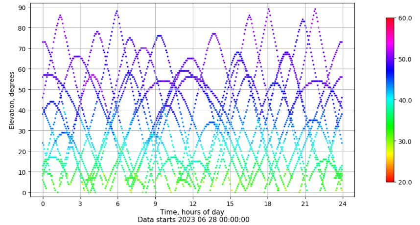
Time-elevation plot for station LALA. Signal to Noise S1C Data file LALA00ESP_R_2023179.xtr
