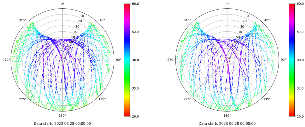
Skyplot for station LALA. Signal to Noise S1C Data file LALA00ESP_R_2023179.xtr Skyplot for station LALA. Signal to Noise S2X Data file LALA00ESP_R_2023179.xtr
