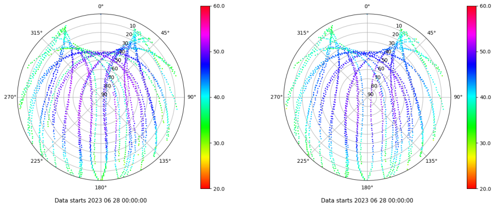
Skyplot for station LALA. Signal to Noise S1C Data file LALA00ESP_R_2023179.xtr Skyplot for station LALA. Signal to Noise S2C Data file LALA00ESP_R_2023179.xtr
