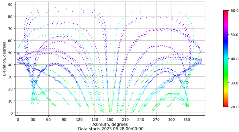
Azimuth-elevation plot for station LALA. Signal to Noise S1C Data file LALA00ESP_R_2023179.xtr
