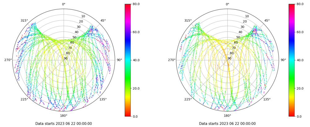
Skyplot for station LALA. Parameter M1C Data file LALA00ESP_R_2023173.xtr Skyplot for station LALA. Parameter M2X Data file LALA00ESP_R_2023173.xtr
