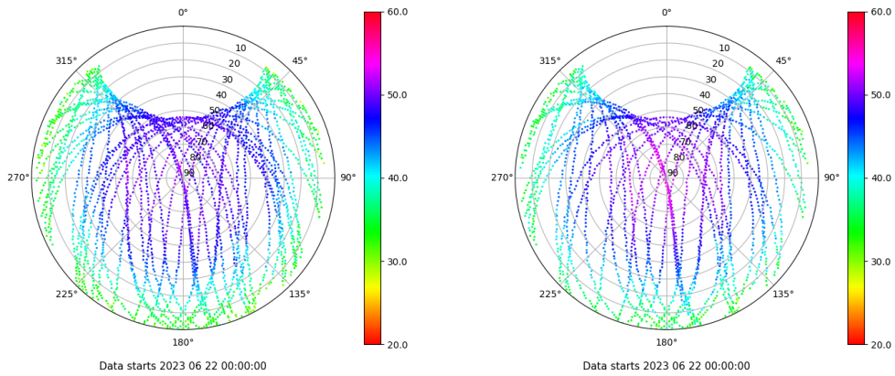
Skyplot for station LALA. Signal to Noise S1C Data file LALA00ESP_R_2023173.xtr Skyplot for station LALA. Signal to Noise S2X Data file LALA00ESP_R_2023173.xtr
