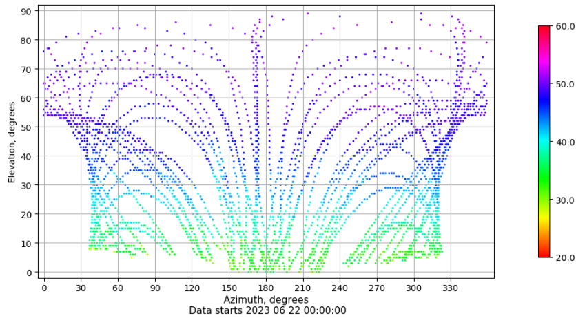
Azimuth-elevation plot for station LALA. Signal to Noise S1C Data file LALA00ESP_R_2023173.xtr
