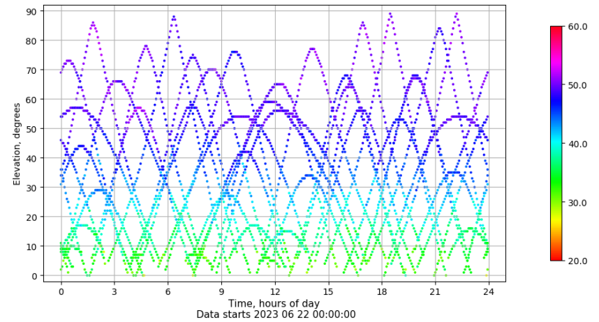
Time-elevation plot for station LALA. Signal to Noise S1C Data file LALA00ESP_R_2023173.xtr
