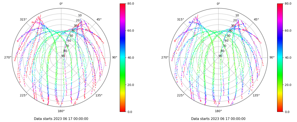
Skyplot for station LALA. Parameter M1C Data file LALA00ESP_R_2023168.xtr Skyplot for station LALA. Parameter M2C Data file LALA00ESP_R_2023168.xtr
