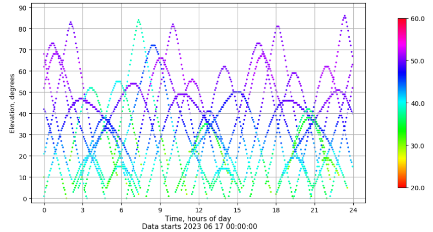
Time-elevation plot for station LALA. Signal to Noise S1C Data file LALA00ESP_R_2023168.xtr
