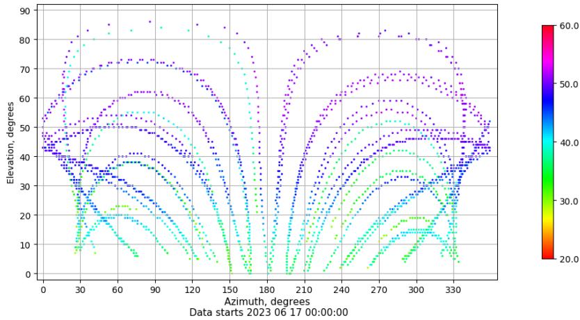
Azimuth-elevation plot for station LALA. Signal to Noise S1C Data file LALA00ESP_R_2023168.xtr
