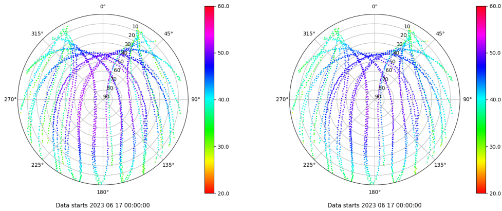
Skyplot for station LALA. Signal to Noise S1C Data file LALA00ESP_R_2023168.xtr Skyplot for station LALA. Signal to Noise S2C Data file LALA00ESP_R_2023168.xtr
