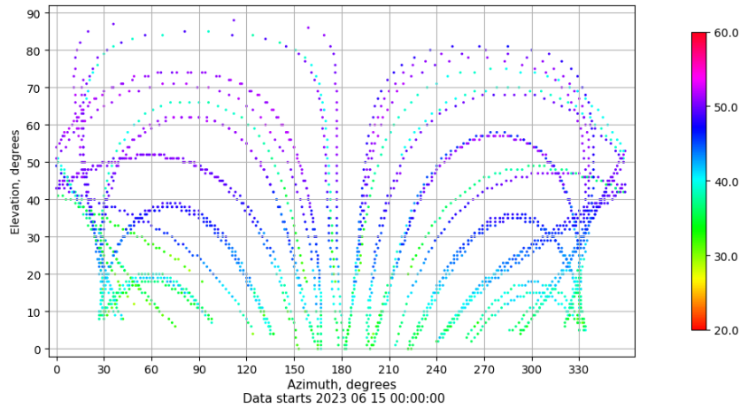
Azimuth-elevation plot for station LALA. Signal to Noise S1C Data file LALA00ESP_R_2023166.xtr
