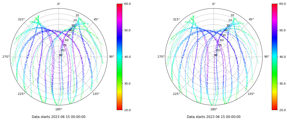
Skyplot for station LALA. Signal to Noise S1C Data file LALA00ESP_R_2023166.xtr Skyplot for station LALA. Signal to Noise S2C Data file LALA00ESP_R_2023166.xtr
