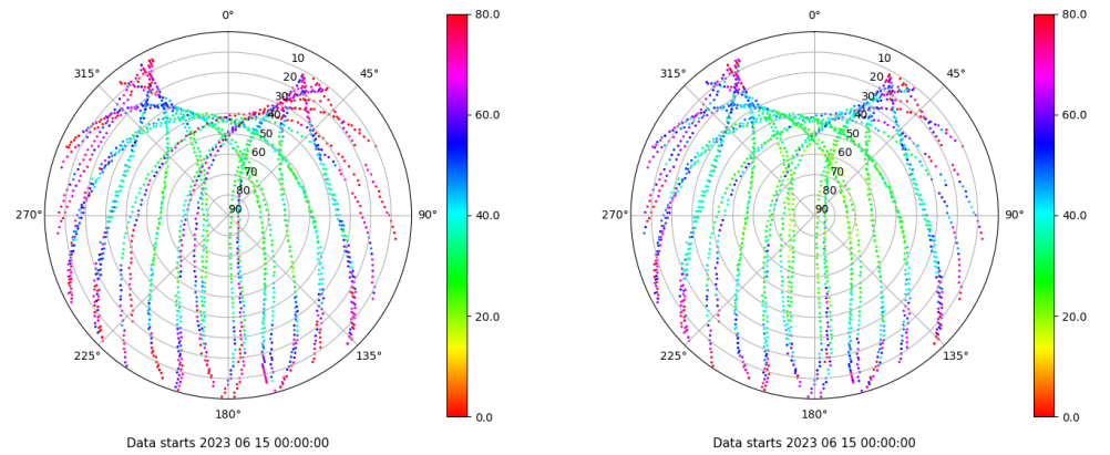
Skyplot for station LALA. Parameter M1C Data file LALA00ESP_R_2023166.xtr Skyplot for station LALA. Parameter M2C Data file LALA00ESP_R_2023166.xtr
