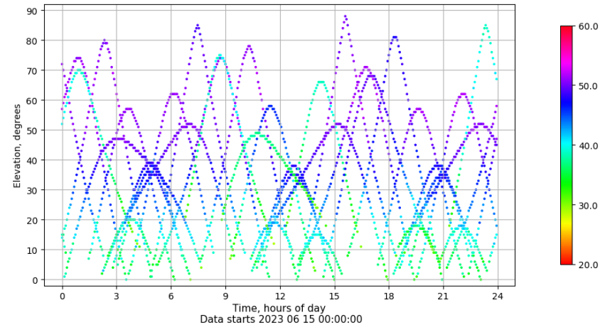
Time-elevation plot for station LALA. Signal to Noise S1C Data file LALA00ESP_R_2023166.xtr
