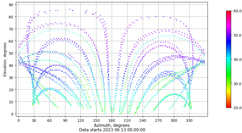
Azimuth-elevation plot for station LALA. Signal to Noise S1C Data file LALA00ESP_R_2023164.xtr
