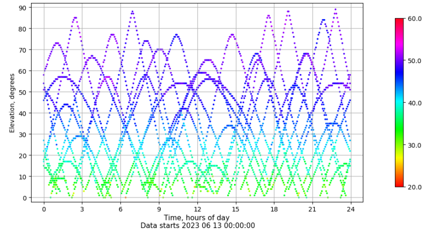
Time-elevation plot for station LALA. Signal to Noise S1C Data file LALA00ESP_R_2023164.xtr
