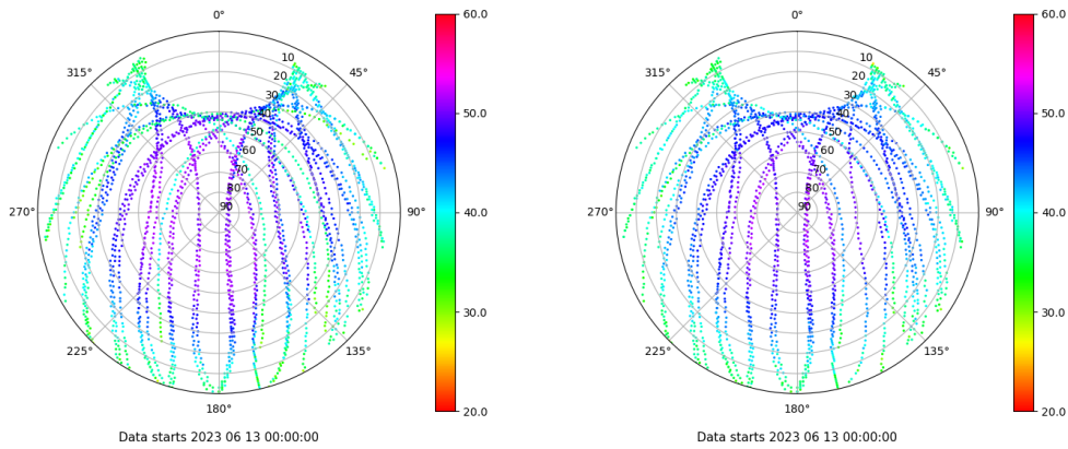
Skyplot for station LALA. Signal to Noise S1C Data file LALA00ESP_R_2023164.xtr Skyplot for station LALA. Signal to Noise S2C Data file LALA00ESP_R_2023164.xtr
