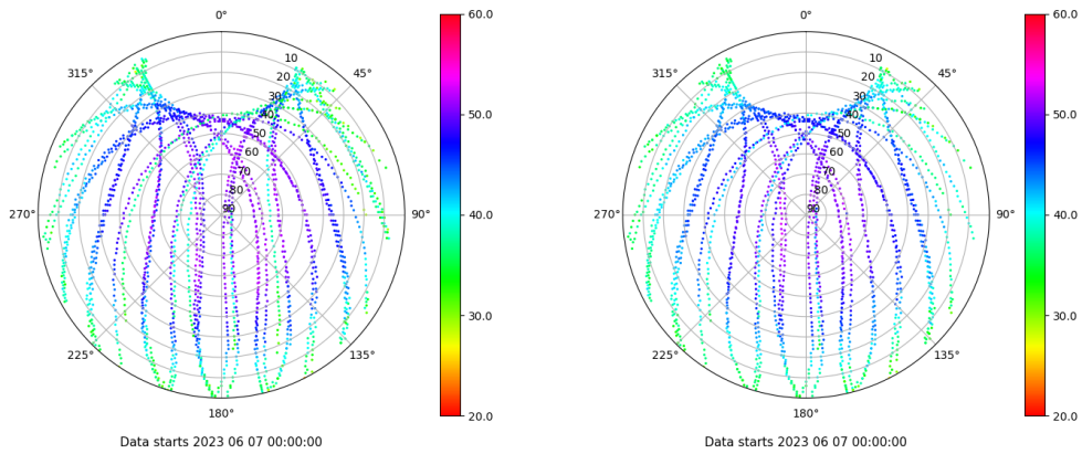
Skyplot for station LALA. Signal to Noise S1C Data file LALA00ESP_R_2023158.xtr Skyplot for station LALA. Signal to Noise S2C Data file LALA00ESP_R_2023158.xtr
