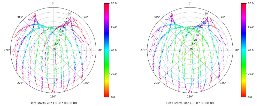
Skyplot for station LALA. Parameter M1C Data file LALA00ESP_R_2023158.xtr Skyplot for station LALA. Parameter M2C Data file LALA00ESP_R_2023158.xtr
