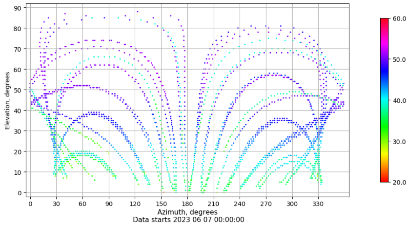
Azimuth-elevation plot for station LALA. Signal to Noise S1C Data file LALA00ESP_R_2023158.xtr
