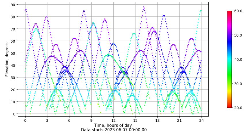
Time-elevation plot for station LALA. Signal to Noise S1C Data file LALA00ESP_R_2023158.xtr
