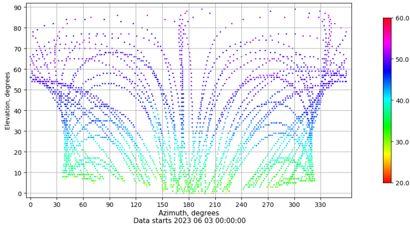
Azimuth-elevation plot for station LALA. Signal to Noise S1C Data file LALA00ESP_R_2023154.xtr
