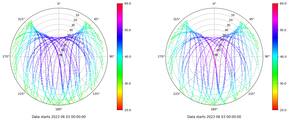
Skyplot for station LALA. Signal to Noise S1C Data file LALA00ESP_R_2023154.xtr Skyplot for station LALA. Signal to Noise S2X Data file LALA00ESP_R_2023154.xtr
