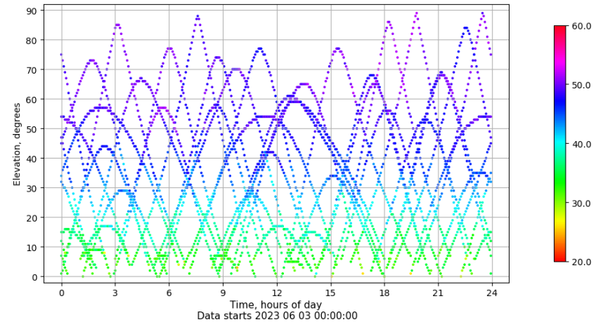
Time-elevation plot for station LALA. Signal to Noise S1C Data file LALA00ESP_R_2023154.xtr
