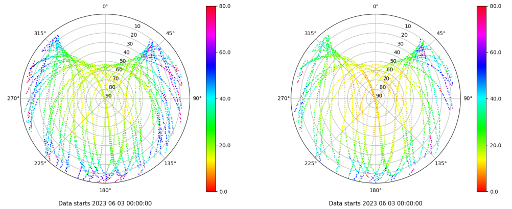
Skyplot for station LALA. Parameter M1C Data file LALA00ESP_R_2023154.xtr Skyplot for station LALA. Parameter M2X Data file LALA00ESP_R_2023154.xtr
