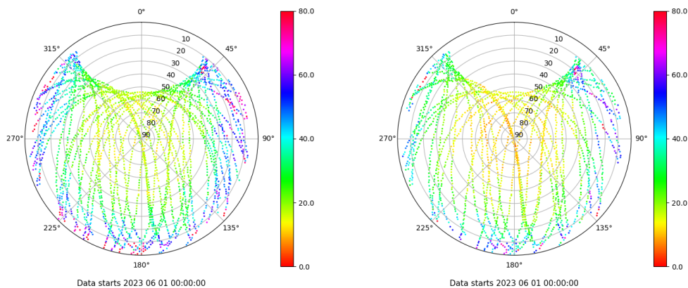
Skyplot for station LALA. Parameter M1C Data file LALA00ESP_R_2023152.xtr Skyplot for station LALA. Parameter M2X Data file LALA00ESP_R_2023152.xtr
