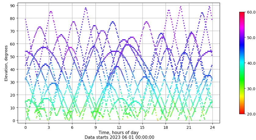
Time-elevation plot for station LALA. Signal to Noise S1C Data file LALA00ESP_R_2023152.xtr
