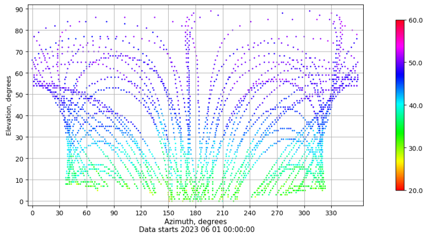
Azimuth-elevation plot for station LALA. Signal to Noise S1C Data file LALA00ESP_R_2023152.xtr
