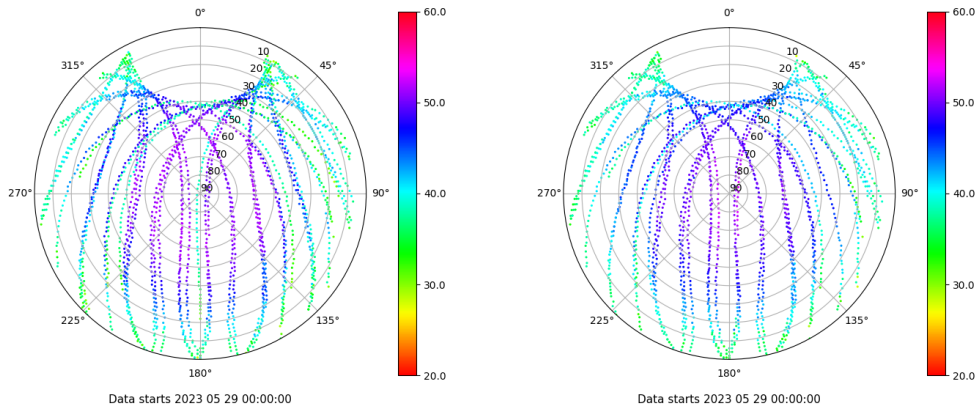
Skyplot for station LALA. Signal to Noise S1C Data file LALA00ESP_R_2023149.xtr Skyplot for station LALA. Signal to Noise S2C Data file LALA00ESP_R_2023149.xtr
