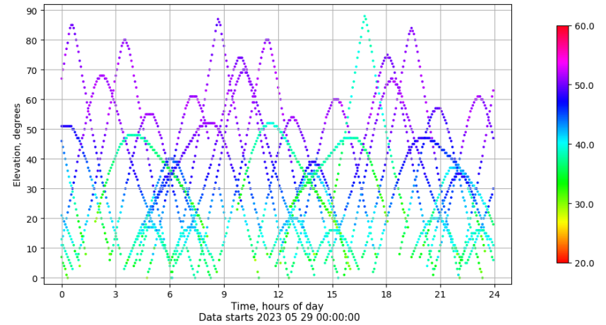
Time-elevation plot for station LALA. Signal to Noise S1C Data file LALA00ESP_R_2023149.xtr
