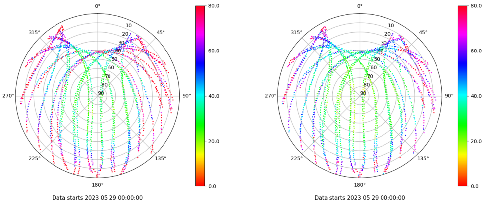
Skyplot for station LALA. Parameter M1C Data file LALA00ESP_R_2023149.xtr Skyplot for station LALA. Parameter M2C Data file LALA00ESP_R_2023149.xtr
