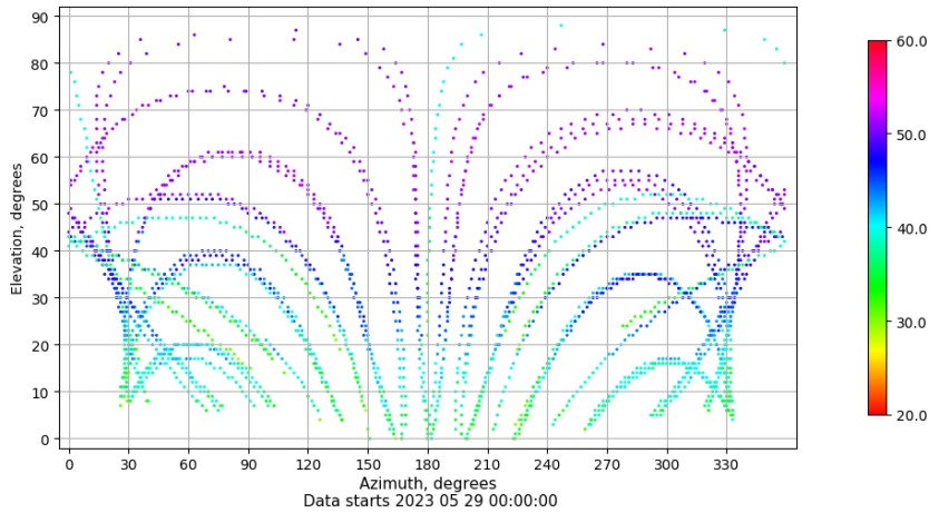
Azimuth-elevation plot for station LALA. Signal to Noise S1C Data file LALA00ESP_R_2023149.xtr
