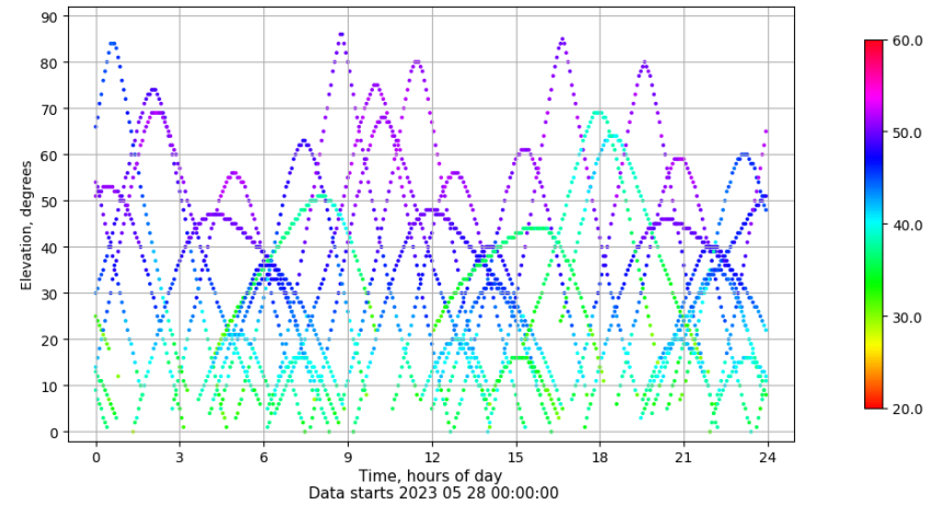
Time-elevation plot for station LALA. Signal to Noise S1C Data file LALA00ESP_R_2023148.xtr
