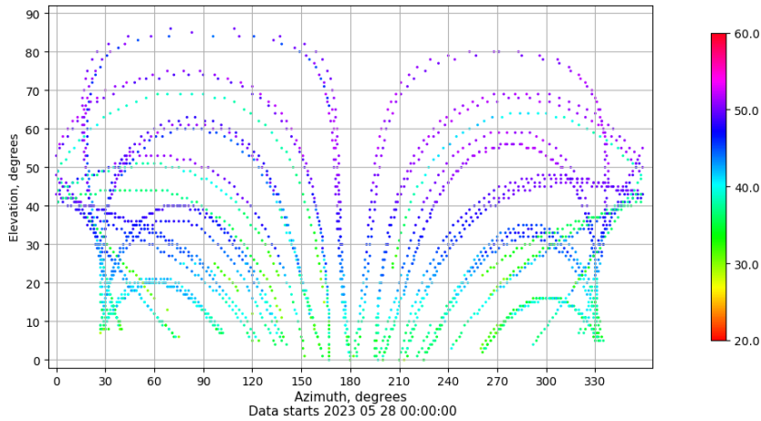
Azimuth-elevation plot for station LALA. Signal to Noise S1C Data file LALA00ESP_R_2023148.xtr
