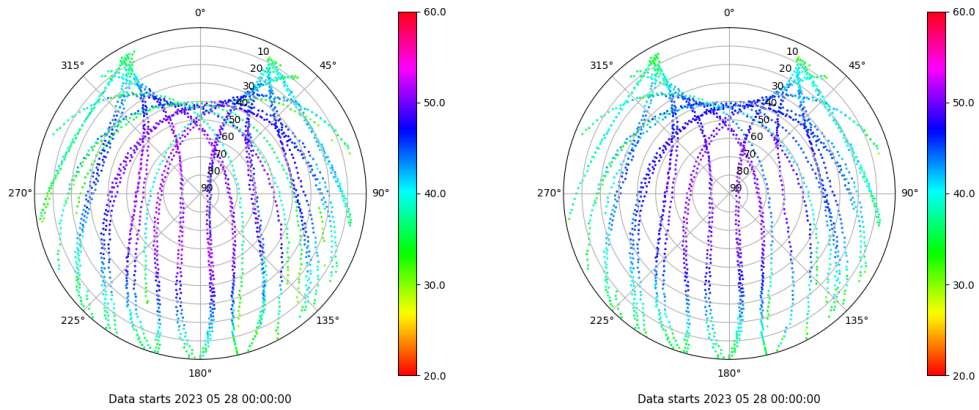
Skyplot for station LALA. Signal to Noise S1C Data file LALA00ESP_R_2023148.xtr Skyplot for station LALA. Signal to Noise S2C Data file LALA00ESP_R_2023148.xtr
