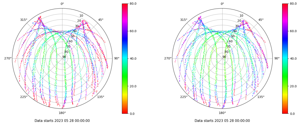
Skyplot for station LALA. Parameter M1C Data file LALA00ESP_R_2023148.xtr Skyplot for station LALA. Parameter M2C Data file LALA00ESP_R_2023148.xtr
