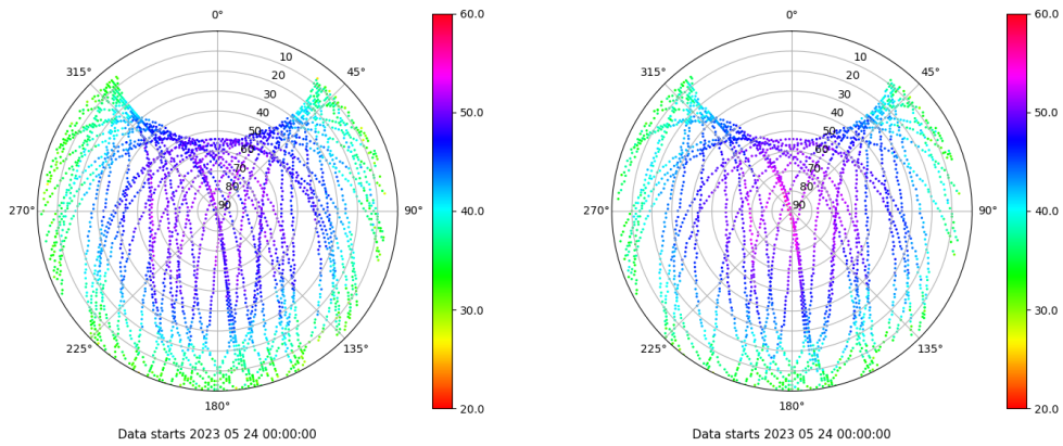
Skyplot for station LALA. Signal to Noise S1C Data file LALA00ESP_R_2023144.xtr Skyplot for station LALA. Signal to Noise S2X Data file LALA00ESP_R_2023144.xtr
