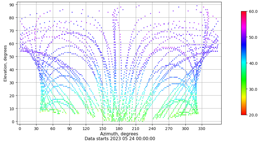
Azimuth-elevation plot for station LALA. Signal to Noise S1C Data file LALA00ESP_R_2023144.xtr
