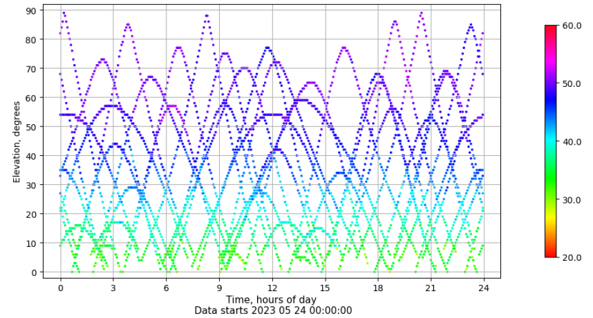
Time-elevation plot for station LALA. Signal to Noise S1C Data file LALA00ESP_R_2023144.xtr
