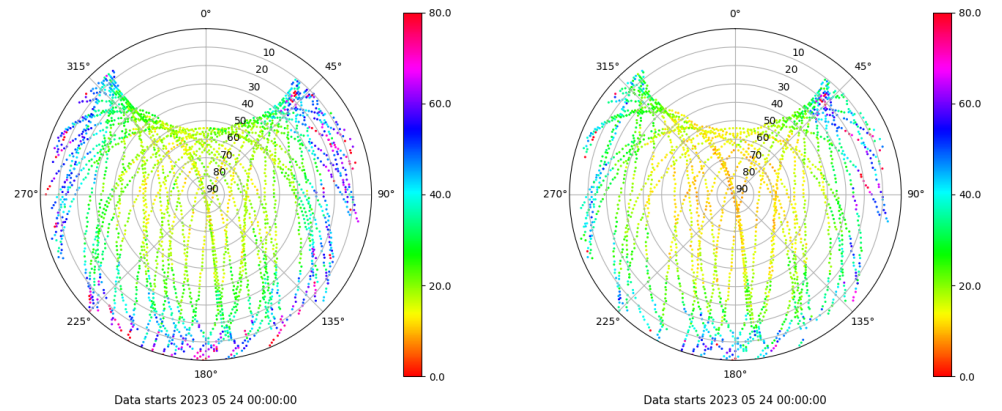
Skyplot for station LALA. Parameter M1C Data file LALA00ESP_R_2023144.xtr Skyplot for station LALA. Parameter M2X Data file LALA00ESP_R_2023144.xtr
