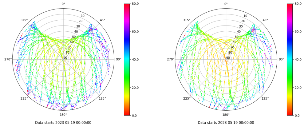
Skyplot for station LALA. Parameter M1C Data file LALA00ESP_R_2023139.xtr Skyplot for station LALA. Parameter M2X Data file LALA00ESP_R_2023139.xtr
