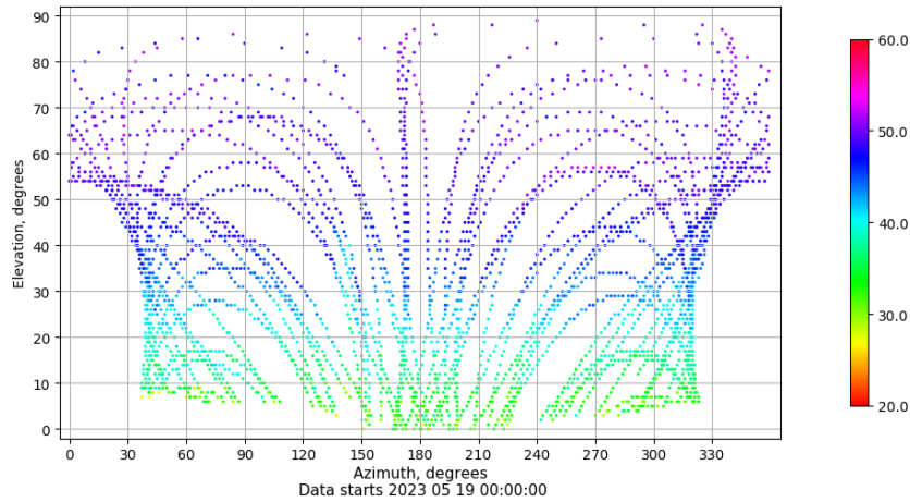
Azimuth-elevation plot for station LALA. Signal to Noise S1C Data file LALA00ESP_R_2023139.xtr
