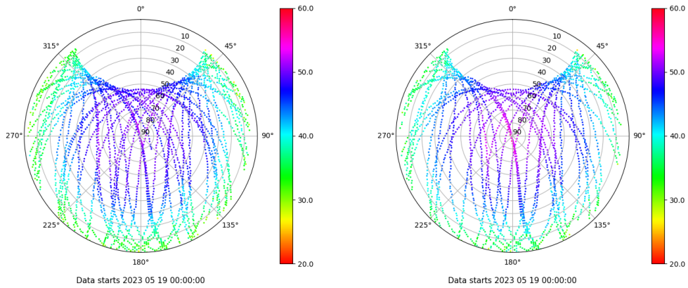
Skyplot for station LALA. Signal to Noise S1C Data file LALA00ESP_R_2023139.xtr Skyplot for station LALA. Signal to Noise S2X Data file LALA00ESP_R_2023139.xtr
