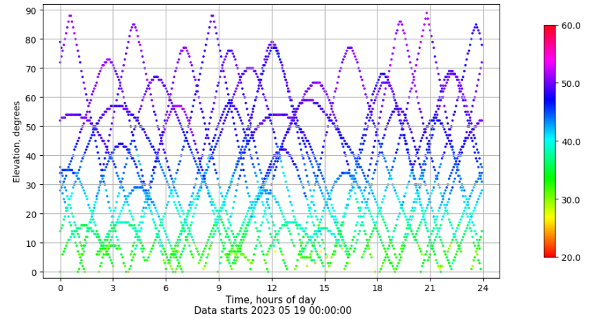
Time-elevation plot for station LALA. Signal to Noise S1C Data file LALA00ESP_R_2023139.xtr
