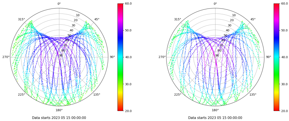
Skyplot for station LALA. Signal to Noise S1C Data file LALA00ESP_R_2023135.xtr Skyplot for station LALA. Signal to Noise S2X Data file LALA00ESP_R_2023135.xtr
