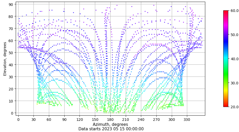
Azimuth-elevation plot for station LALA. Signal to Noise S1C Data file LALA00ESP_R_2023135.xtr
