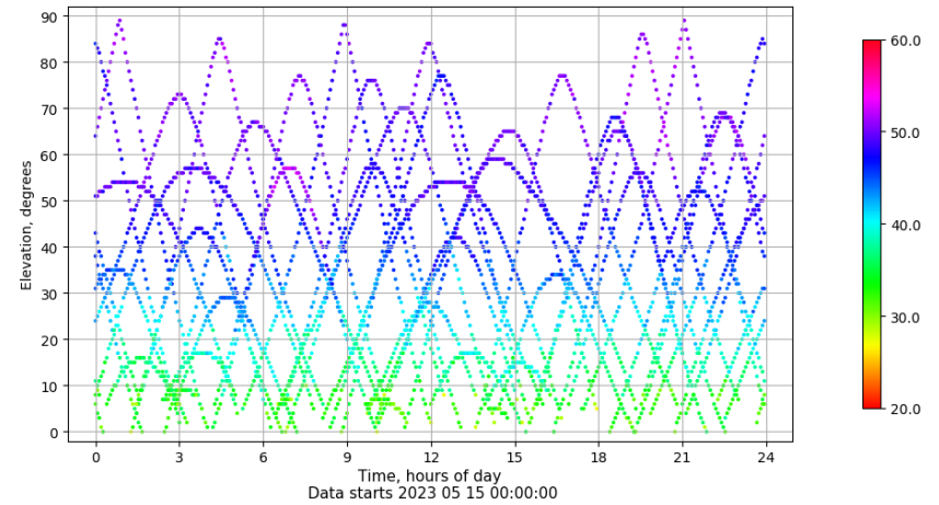
Time-elevation plot for station LALA. Signal to Noise S1C Data file LALA00ESP_R_2023135.xtr
