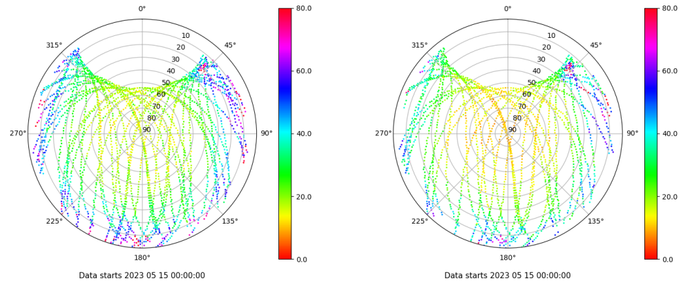
Skyplot for station LALA. Parameter M1C Data file LALA00ESP_R_2023135.xtr Skyplot for station LALA. Parameter M2X Data file LALA00ESP_R_2023135.xtr
