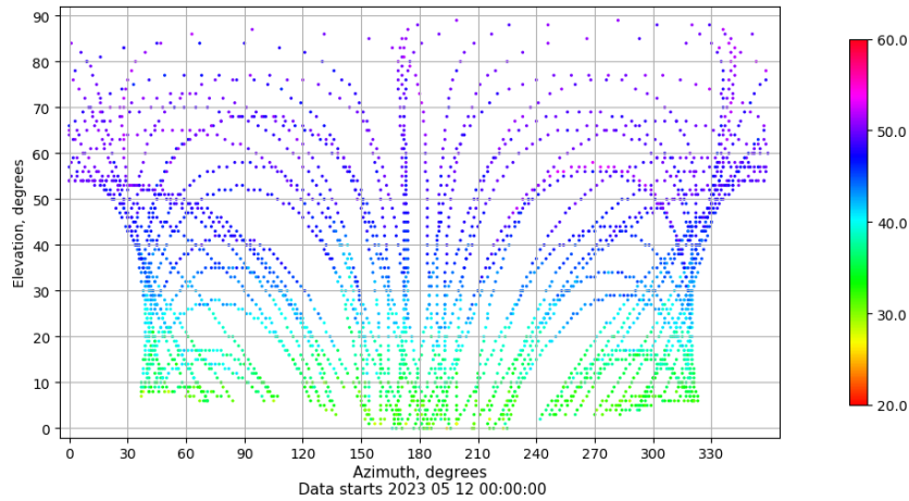
Azimuth-elevation plot for station LALA. Signal to Noise S1C Data file LALA00ESP_R_2023132.xtr
