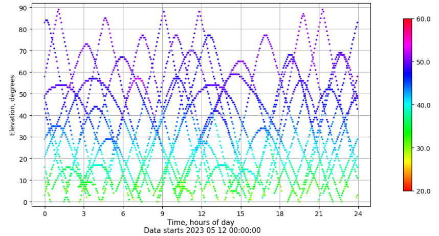
Time-elevation plot for station LALA. Signal to Noise S1C Data file LALA00ESP_R_2023132.xtr
