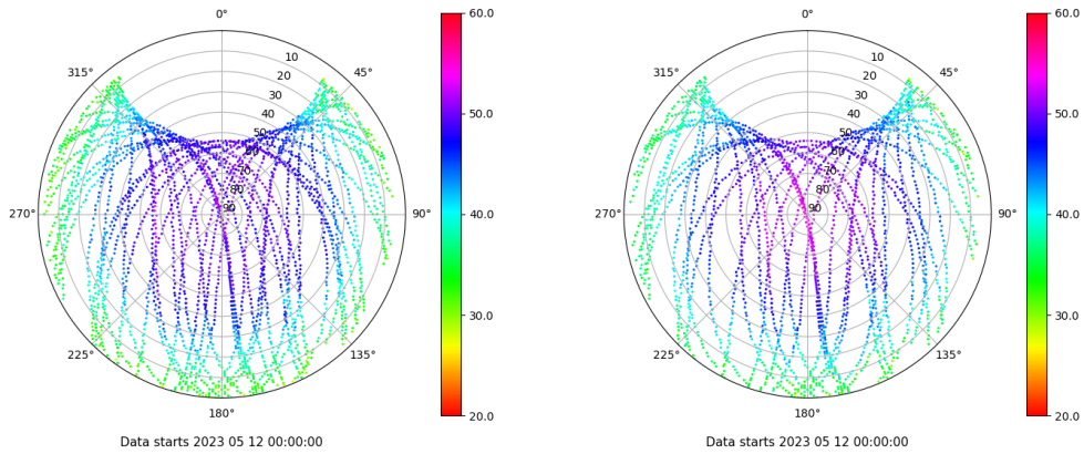
Skyplot for station LALA. Signal to Noise S1C Data file LALA00ESP_R_2023132.xtr Skyplot for station LALA. Signal to Noise S2X Data file LALA00ESP_R_2023132.xtr
