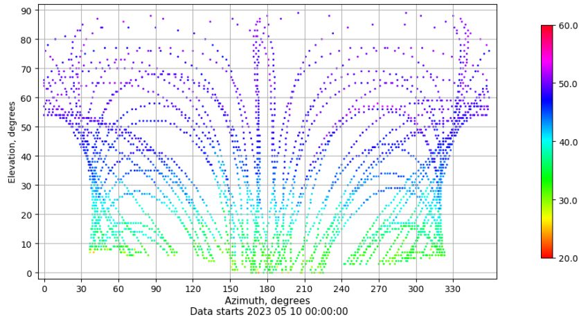
Azimuth-elevation plot for station LALA. Signal to Noise S1C Data file LALA00ESP_R_2023130.xtr
