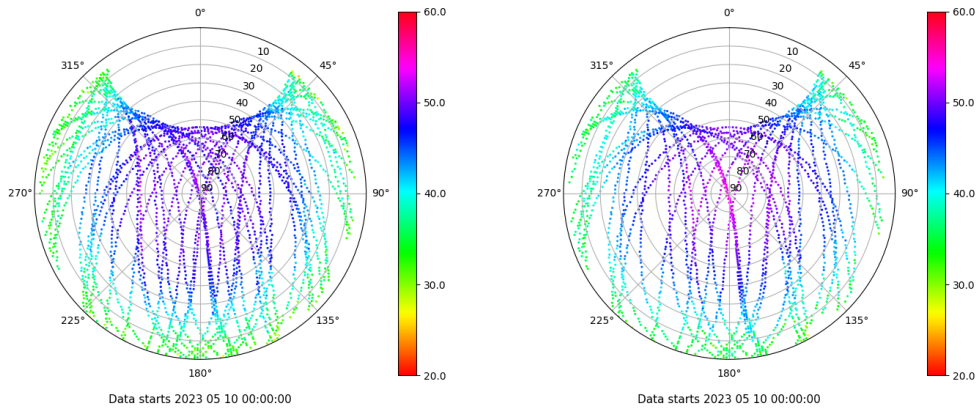
Skyplot for station LALA. Signal to Noise S1C Data file LALA00ESP_R_2023130.xtr Skyplot for station LALA. Signal to Noise S2X Data file LALA00ESP_R_2023130.xtr
