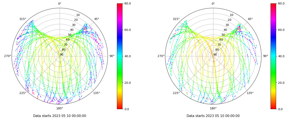
Skyplot for station LALA. Parameter M1C Data file LALA00ESP_R_2023130.xtr Skyplot for station LALA. Parameter M2X Data file LALA00ESP_R_2023130.xtr
