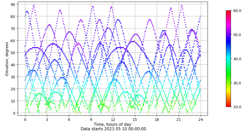
Time-elevation plot for station LALA. Signal to Noise S1C Data file LALA00ESP_R_2023130.xtr
