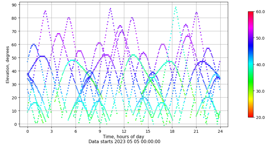
Time-elevation plot for station LALA. Signal to Noise S1C Data file LALA00ESP_R_2023125.xtr
