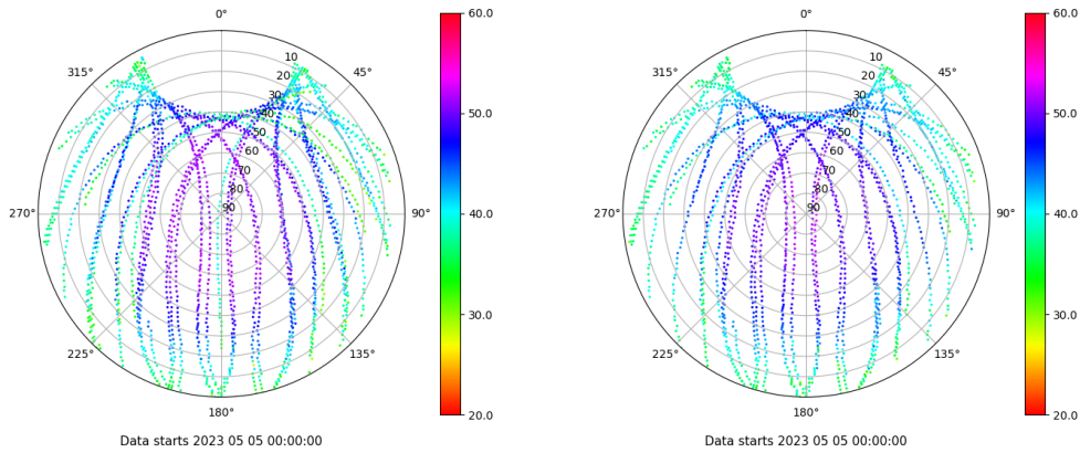
Skyplot for station LALA. Signal to Noise S1C Data file LALA00ESP_R_2023125.xtr Skyplot for station LALA. Signal to Noise S2C Data file LALA00ESP_R_2023125.xtr
