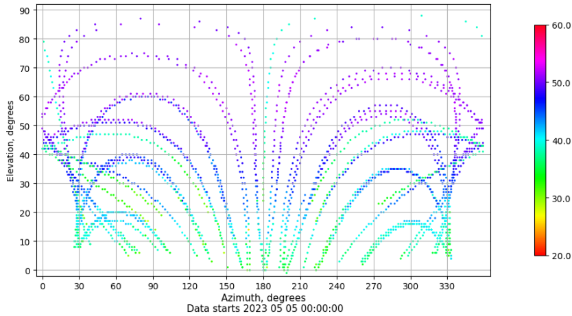
Azimuth-elevation plot for station LALA. Signal to Noise S1C Data file LALA00ESP_R_2023125.xtr
