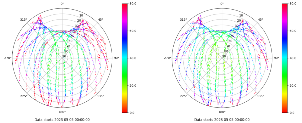
Skyplot for station LALA. Parameter M1C Data file LALA00ESP_R_2023125.xtr Skyplot for station LALA. Parameter M2C Data file LALA00ESP_R_2023125.xtr
