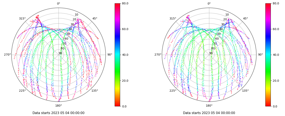
Skyplot for station LALA. Parameter M1C Data file LALA00ESP_R_2023124.xtr Skyplot for station LALA. Parameter M2C Data file LALA00ESP_R_2023124.xtr
