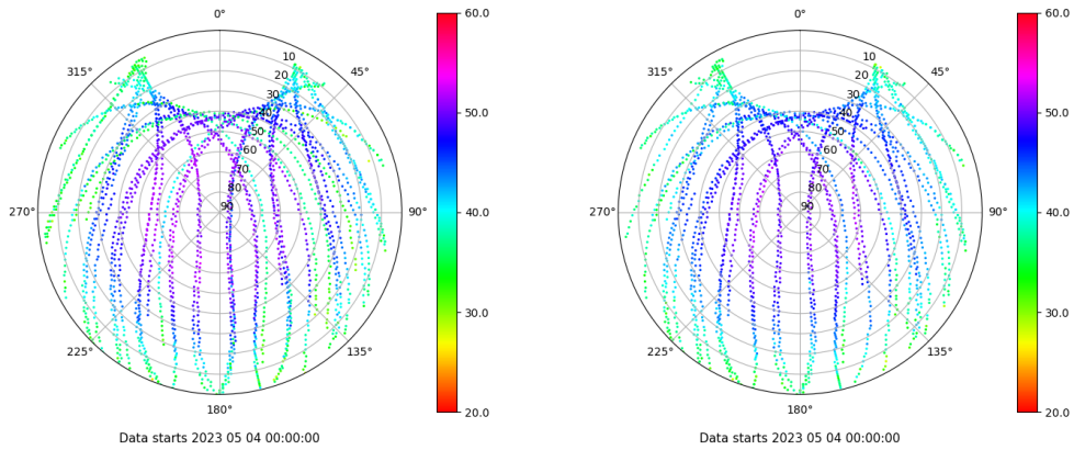
Skyplot for station LALA. Signal to Noise S1C Data file LALA00ESP_R_2023124.xtr Skyplot for station LALA. Signal to Noise S2C Data file LALA00ESP_R_2023124.xtr
