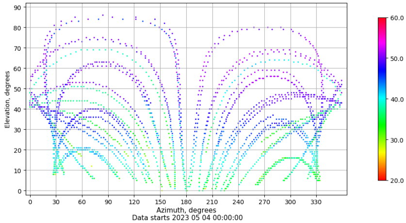
Azimuth-elevation plot for station LALA. Signal to Noise S1C Data file LALA00ESP_R_2023124.xtr
