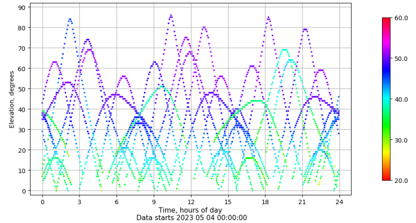
Time-elevation plot for station LALA. Signal to Noise S1C Data file LALA00ESP_R_2023124.xtr
