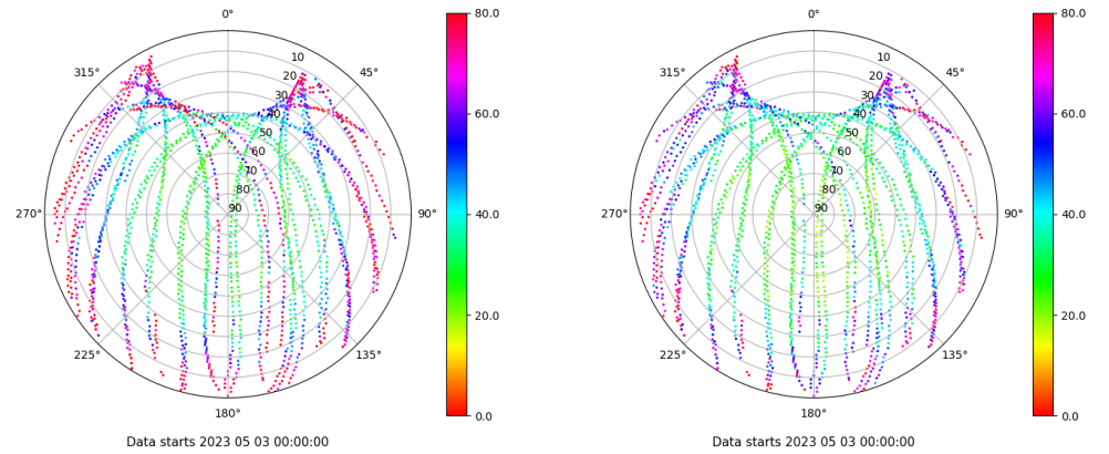
Skyplot for station LALA. Parameter M1C Data file LALA00ESP_R_2023123.xtr Skyplot for station LALA. Parameter M2C Data file LALA00ESP_R_2023123.xtr
