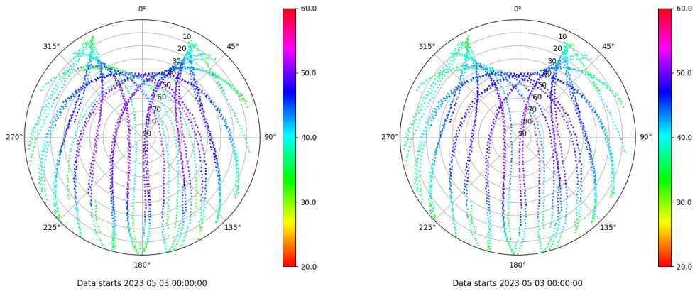
Skyplot for station LALA. Signal to Noise S1C Data file LALA00ESP_R_2023123.xtr Skyplot for station LALA. Signal to Noise S2C Data file LALA00ESP_R_2023123.xtr
