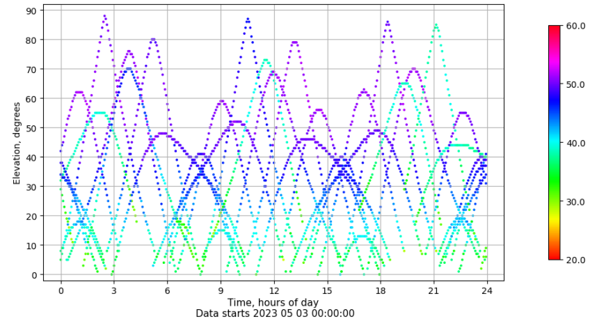
Time-elevation plot for station LALA. Signal to Noise S1C Data file LALA00ESP_R_2023123.xtr
