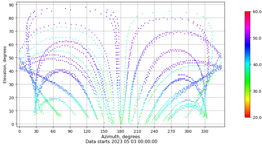
Azimuth-elevation plot for station LALA. Signal to Noise S1C Data file LALA00ESP_R_2023123.xtr
