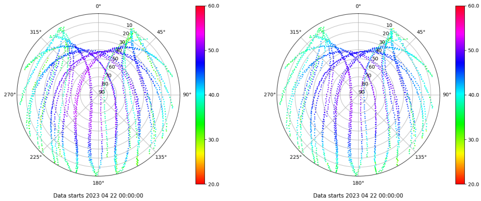
Skyplot for station LALA. Signal to Noise S1C Data file LALA00ESP_R_2023112.xtr Skyplot for station LALA. Signal to Noise S2C Data file LALA00ESP_R_2023112.xtr
