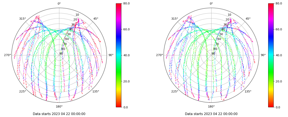
Skyplot for station LALA. Parameter M1C Data file LALA00ESP_R_2023112.xtr Skyplot for station LALA. Parameter M2C Data file LALA00ESP_R_2023112.xtr
