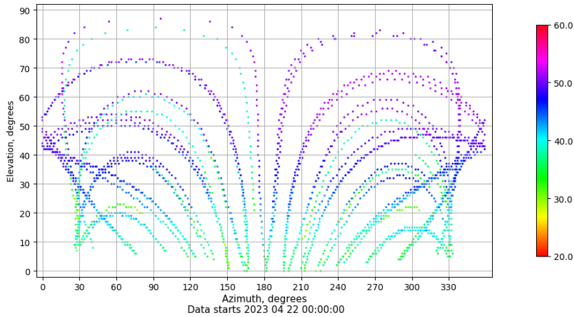
Azimuth-elevation plot for station LALA. Signal to Noise S1C Data file LALA00ESP_R_2023112.xtr
