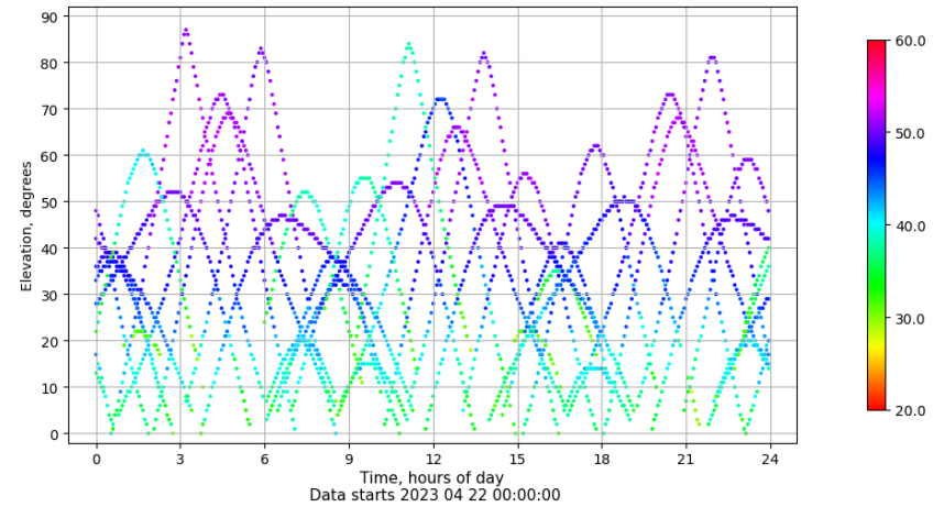
Time-elevation plot for station LALA. Signal to Noise S1C Data file LALA00ESP_R_2023112.xtr
