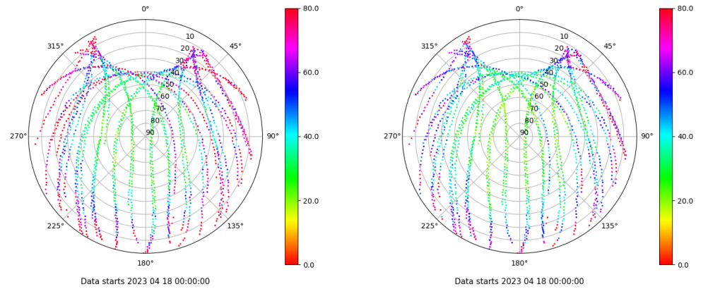
Skyplot for station LALA. Parameter M1C Data file LALA00ESP_R_2023108.xtr Skyplot for station LALA. Parameter M2C Data file LALA00ESP_R_2023108.xtr
