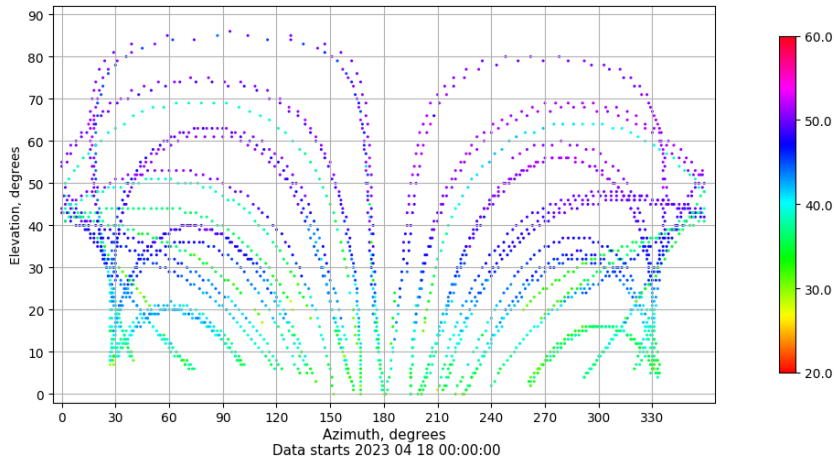
Azimuth-elevation plot for station LALA. Signal to Noise S1C Data file LALA00ESP_R_2023108.xtr
