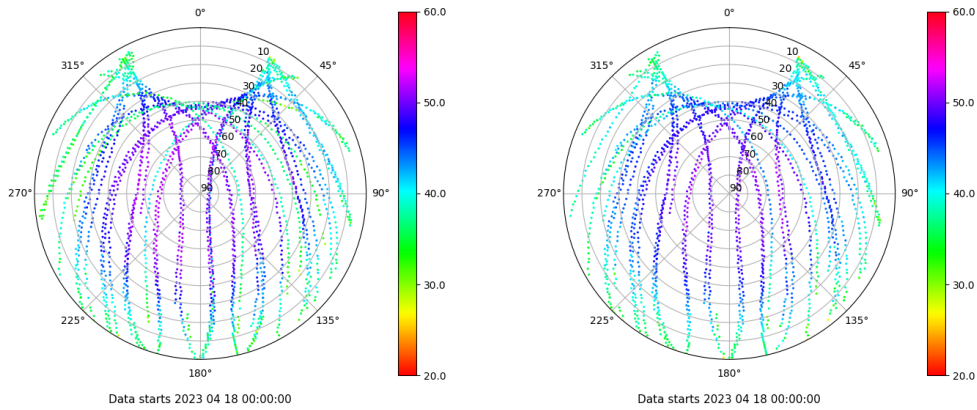
Skyplot for station LALA. Signal to Noise S1C Data file LALA00ESP_R_2023108.xtr Skyplot for station LALA. Signal to Noise S2C Data file LALA00ESP_R_2023108.xtr
