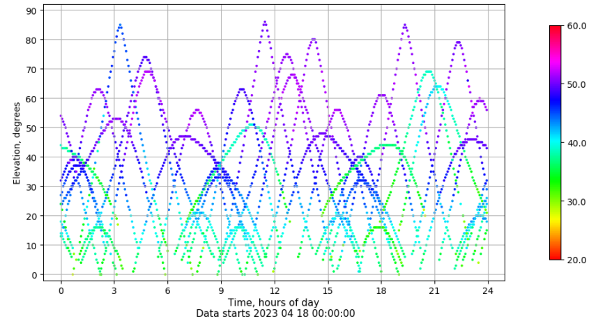
Time-elevation plot for station LALA. Signal to Noise S1C Data file LALA00ESP_R_2023108.xtr
